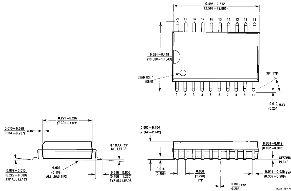
S.O. Package (M) Order Number DM74AS640WM Package Number M20B
