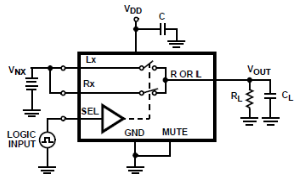
TEST CIRCUIT
