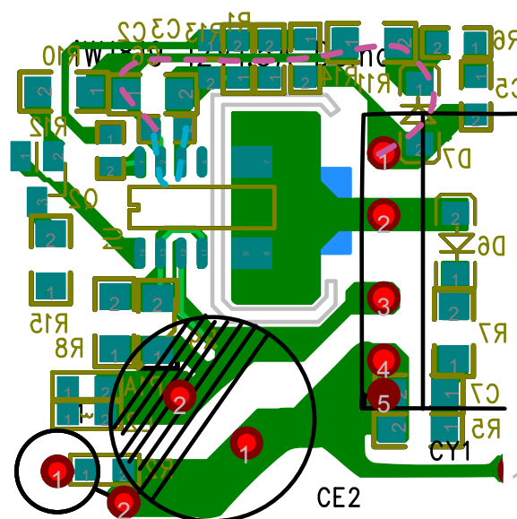
Figure 10.13b : IC Power Supply Layout Path
