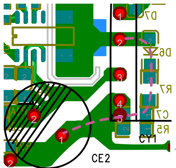
Figure 10.12b : Snubber Circuit Layout Path
