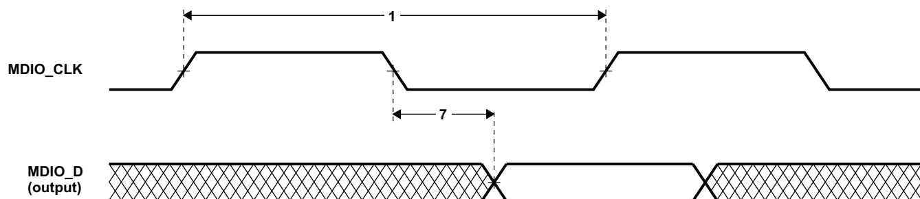
Figure 6-26. MDIO Output Timing
