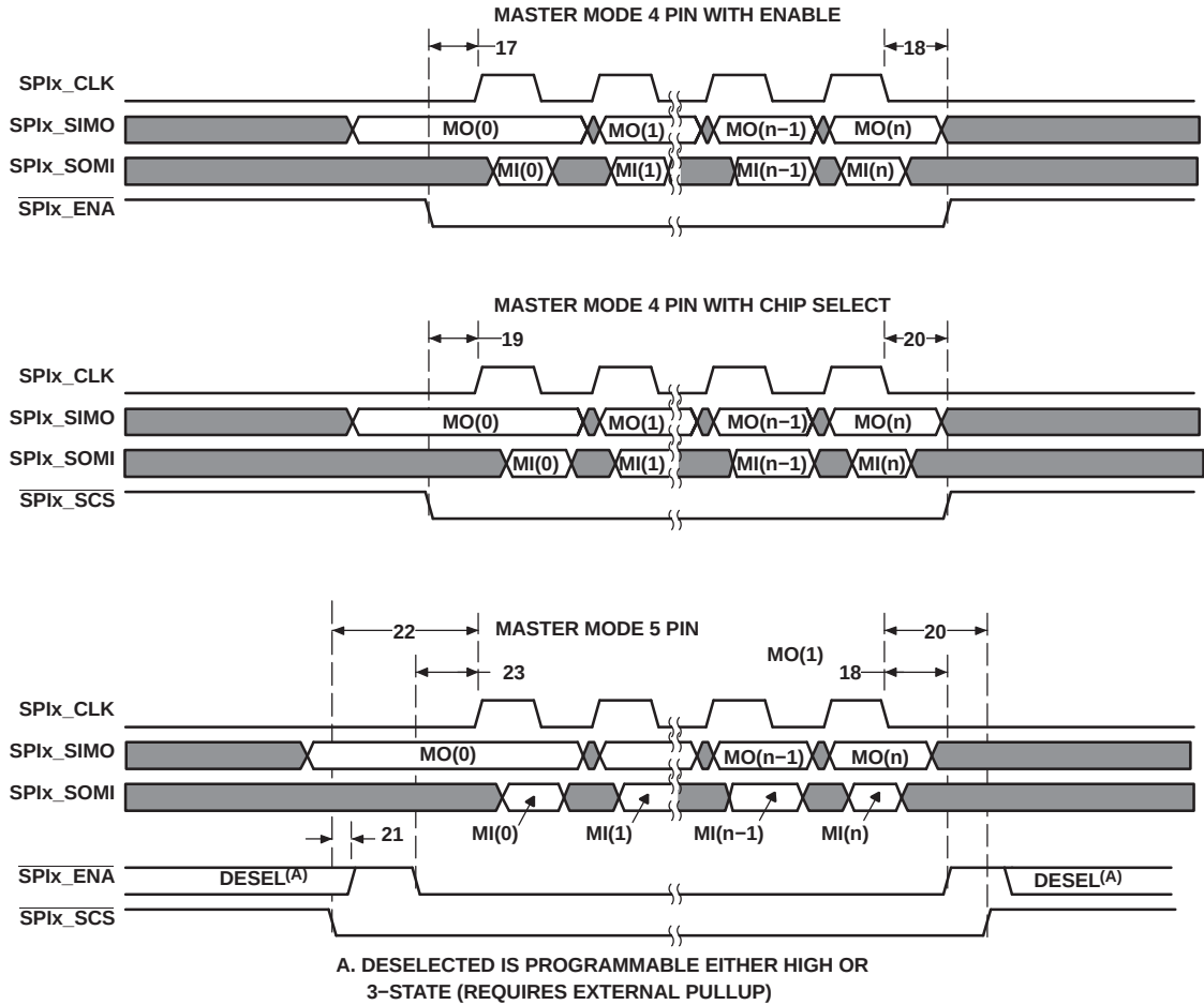
Figure 6-34. SPI Timings—Master Mode (4-Pin and 5-Pin)
