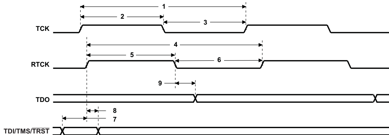
Figure 6-51. JTAG Test-Port Timing
