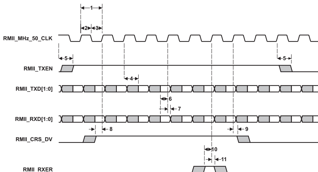
Figure 6-24. RMII Timing Diagram
