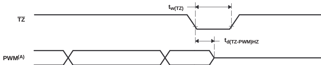
Figure 6-40. PWM Hi-Z Characteristics
