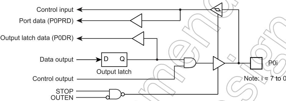
Figure 5-2 Port P0
