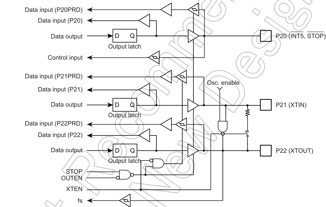
Figure 5-4 Port P2
