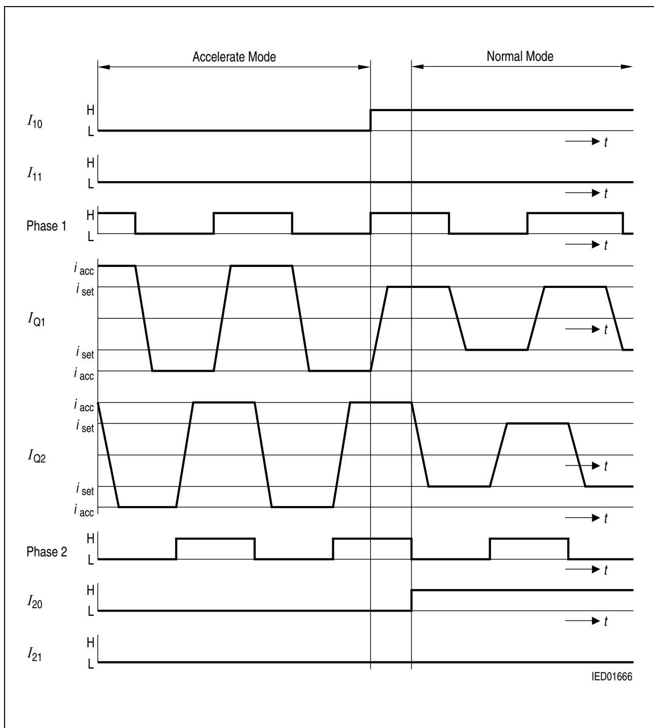
Figure 7 Full-Step Operation
