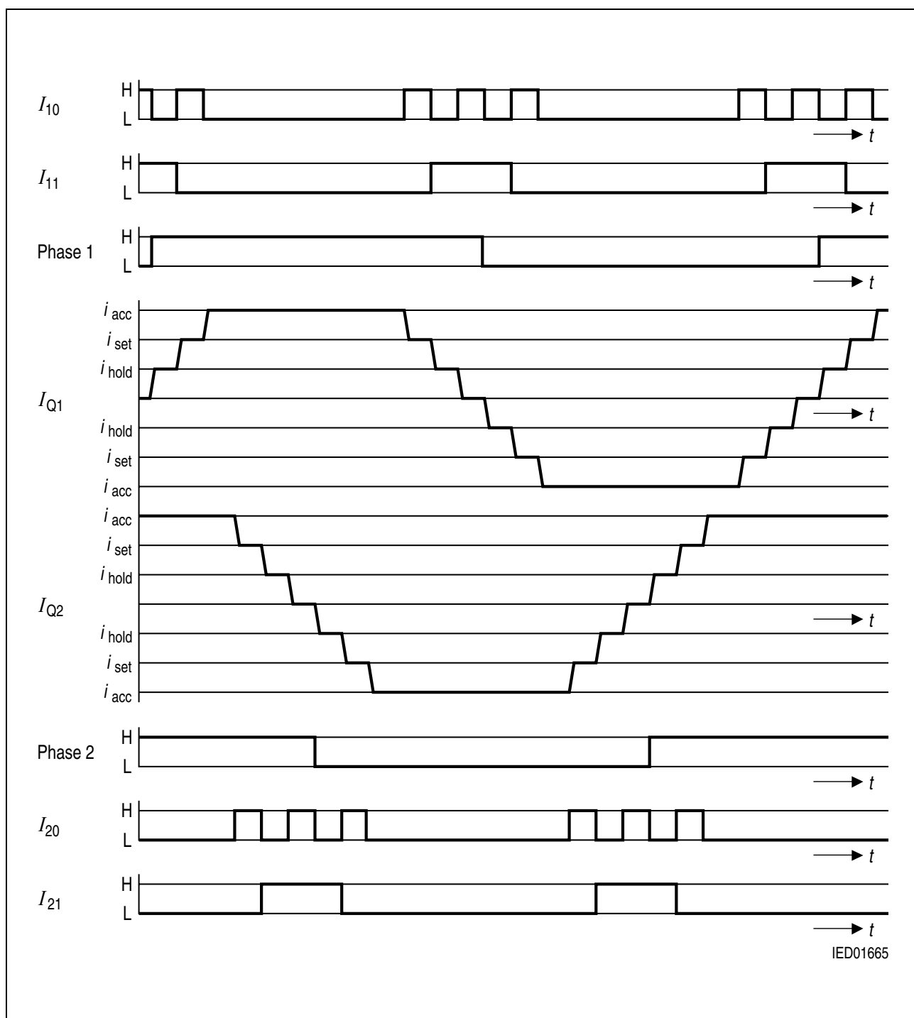
Figure 10 Mini-Step Operation
