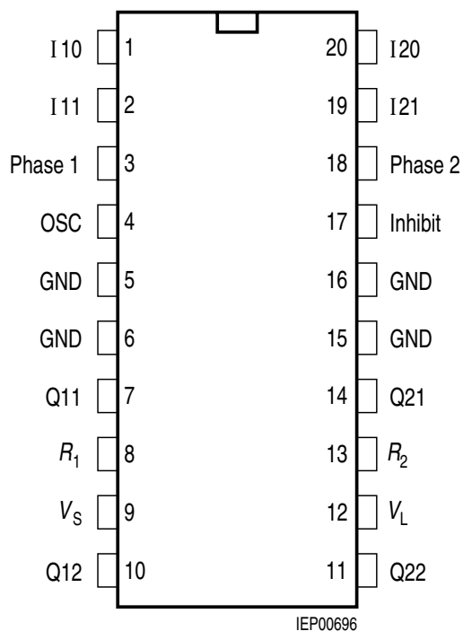
Figure 1 Pin Configuration TCA 3727 (top view)
