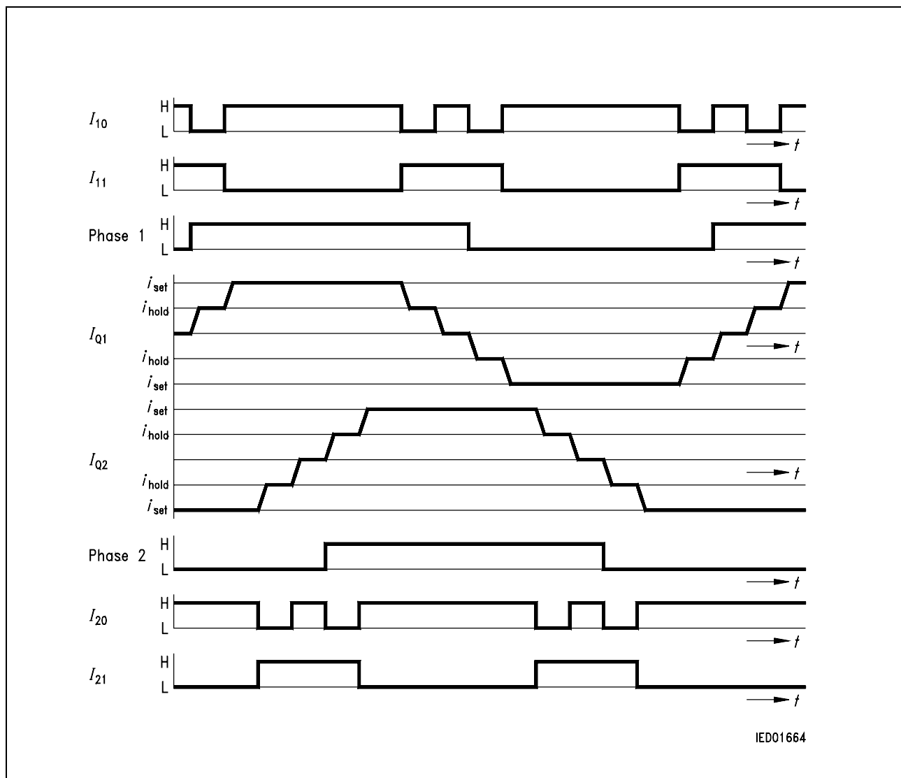
Figure 9 Quarter-Step Operation
