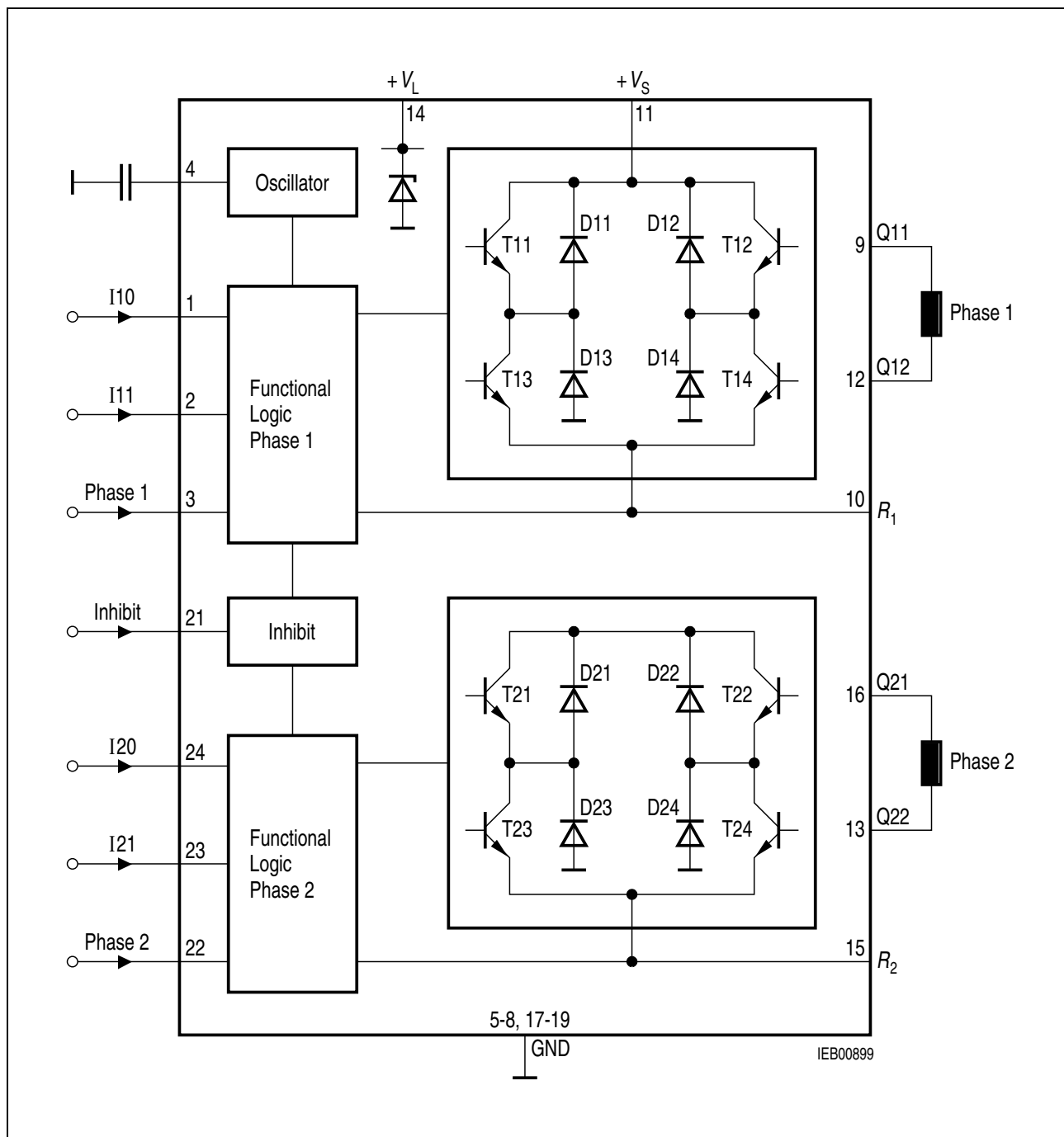
Figure 4 Block Diagram TCA 3727 G
