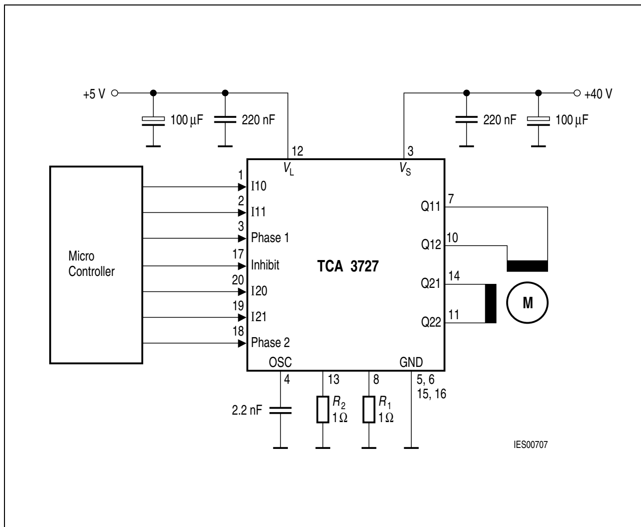
Figure 6 Application Circuit
