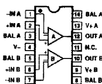
14-PIN HERMETIC DIP (Y-Suffix) OP-04
