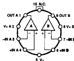
TO-100 (K-Suffix) OP-04
