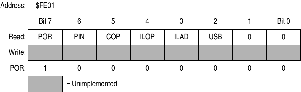
Figure 9-20. SIM Reset Status Register (SRSR)
