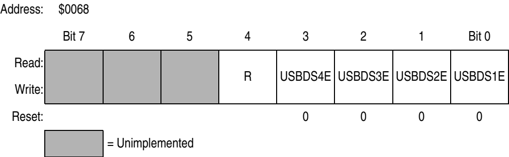
Figure 19-20. Port E Control Register (PECR)
