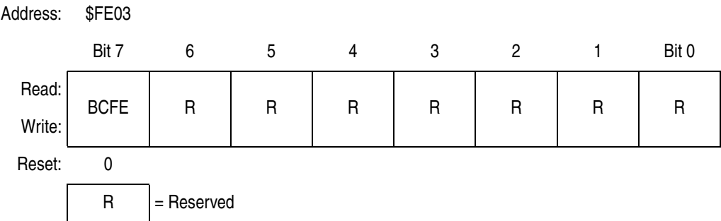
Figure 9-21. SIM Break Flag Control Register (SBFCR)
