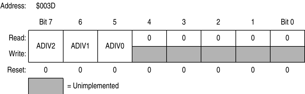
Figure 13-5. ADC Input Clock Register (ADICLK)
