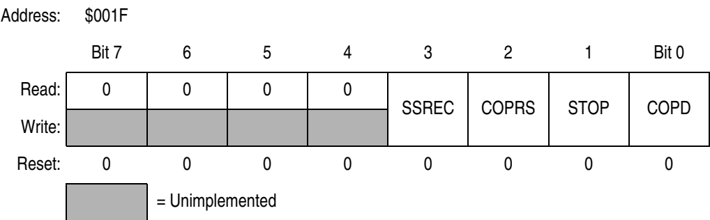
Figure 22-2. Configuration Register (CONFIG)
