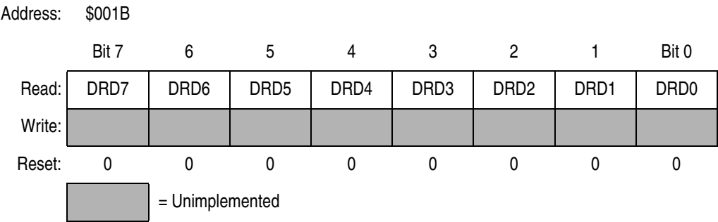
Figure 16-8. DDC Data Receive Register (DDCDRR)
