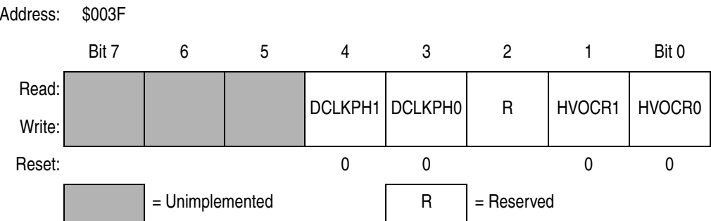
Figure 8-6. H&V Sync Output Control Register (HVOCR)
