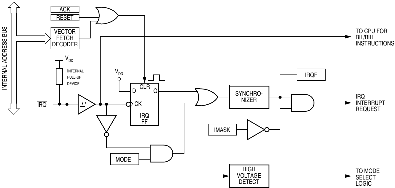
Figure 20-1. IRQ Module Block Diagram
