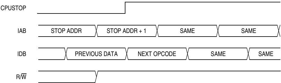
Figure 9-17. Stop Mode Entry Timing
