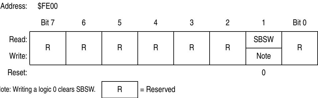
Figure 9-19. SIM Break Status Register (SBSR)
