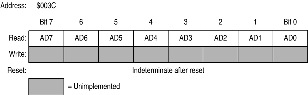
Figure 13-4. ADC Data Register (ADR)
