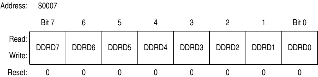
Figure 19-14. Data Direction Register D (DDRD)
