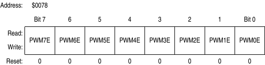
Figure 12-3. PWM Control Register (PWMCR)
