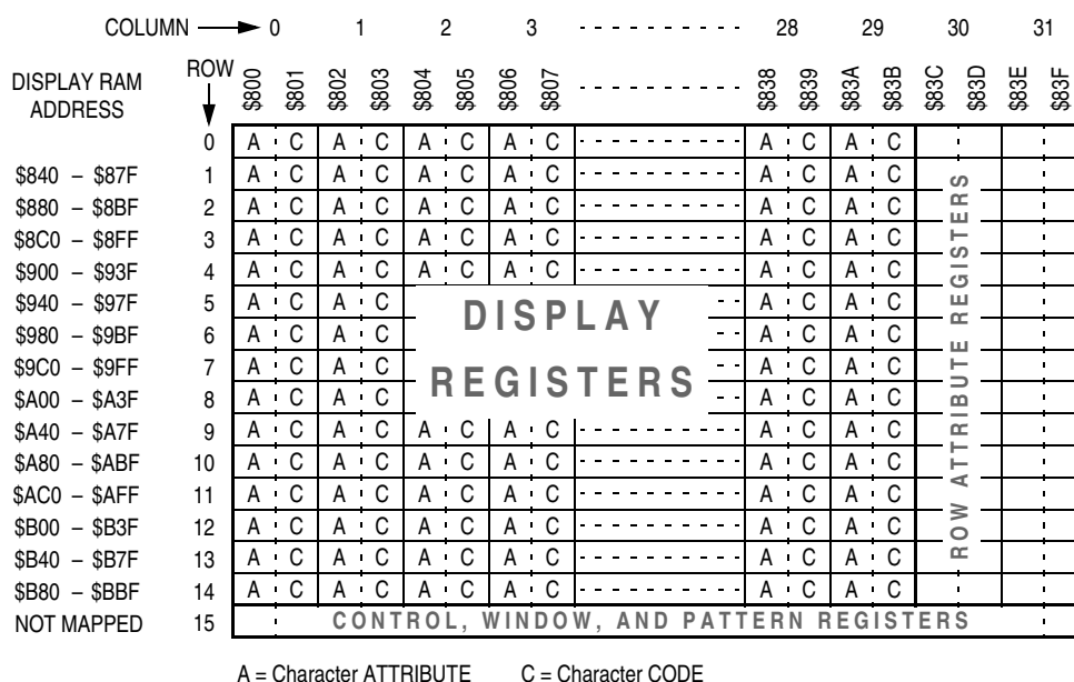
Figure 18-4. Memory Map of OSD Registers
