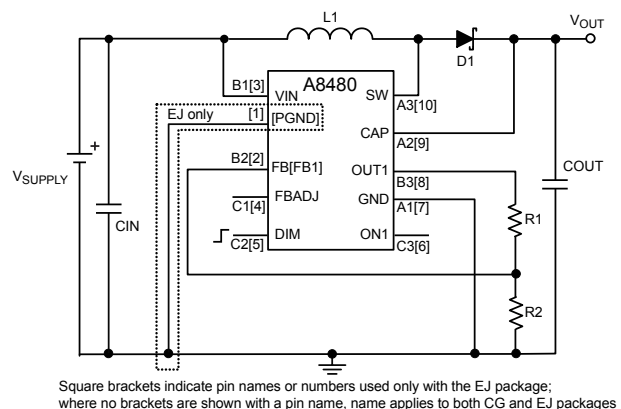
Figure 2. The A8480 used as a general boost
