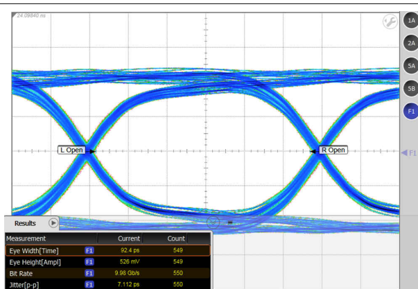
Figure 9-6. 10 Gbps PRBS-7 Signals Through a Typical TMUXHS4212 Channel in TI Evaluation Board
