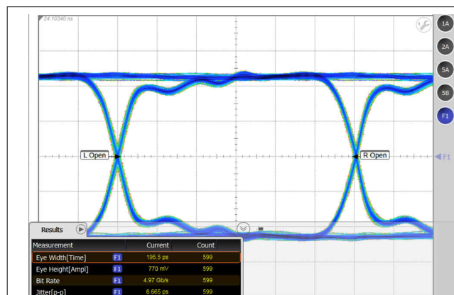
Figure 9-3. 5 Gbps PRBS-7 Signals Through Calibration Traces in TI Evaluation Board
