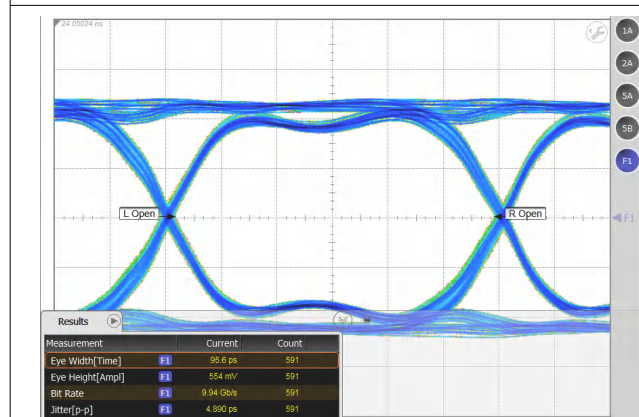
Figure 9-5. 10 Gbps PRBS-7 Signals Through Calibration Traces in TI Evaluation Board
