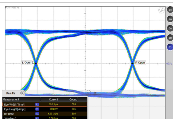
Figure 9-4. 5 Gbps PRBS-7 Signals Through a Typical TMUXHS4212 Channel in TI Evaluation Board
