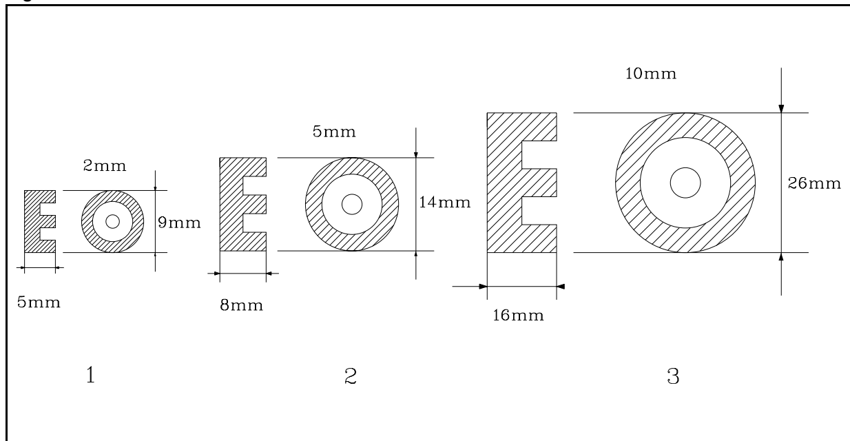
Figure 4. Detection distance
