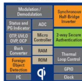
IDTP9030 Transmitter
