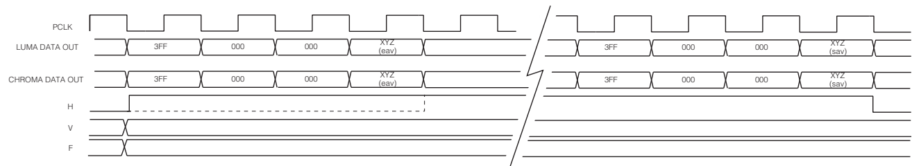
H:V:F TIMING - HD 20-BIT INPUT MODE
