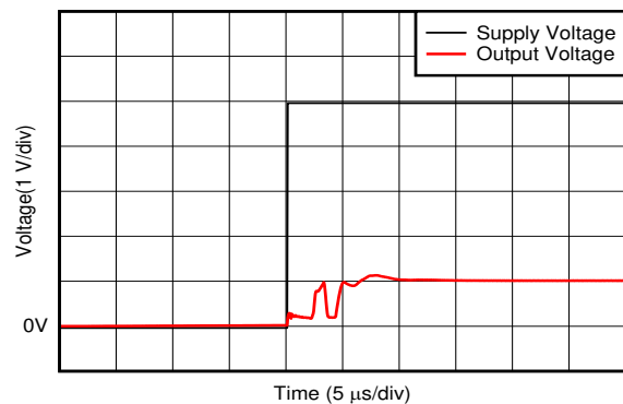
Figure 7-25. Start-Up Response
