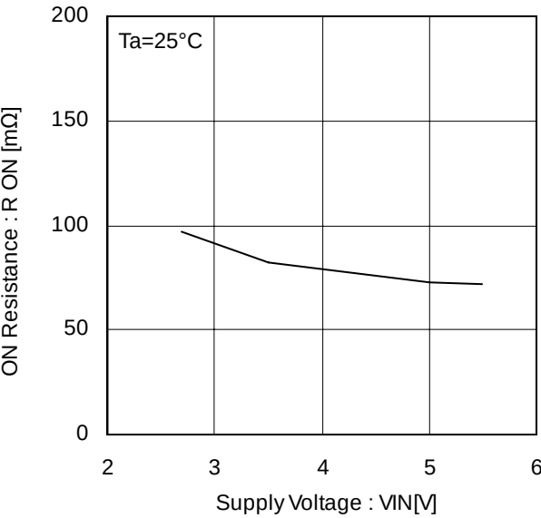
Figure 10. On-resistance
