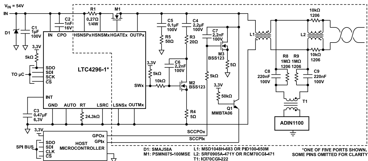
Figure 62. IEEE 802.3cq Class 14 PSE
