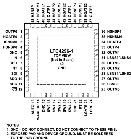
Figure 3. Pin Configuration
