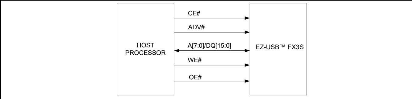
Figure 8 ADMux memory interface
