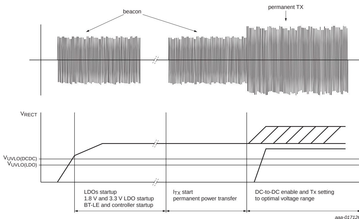
Fig 9. NX2A4WP start-up sequence
