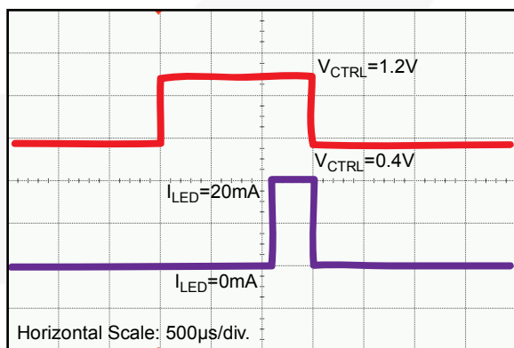
Figure 14. Active Modes Delay
