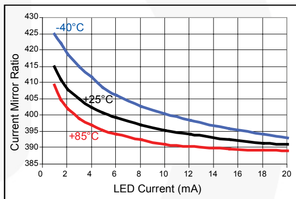
Figure 12. Current Mirror Ratio vs. Output Current
