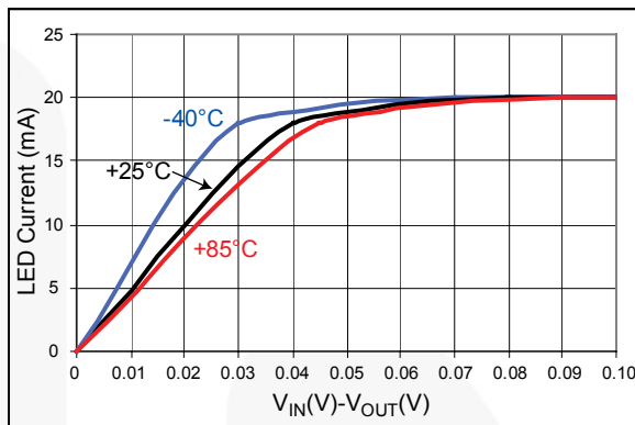
Figure 10. LED Current vs. Headroom Voltage
