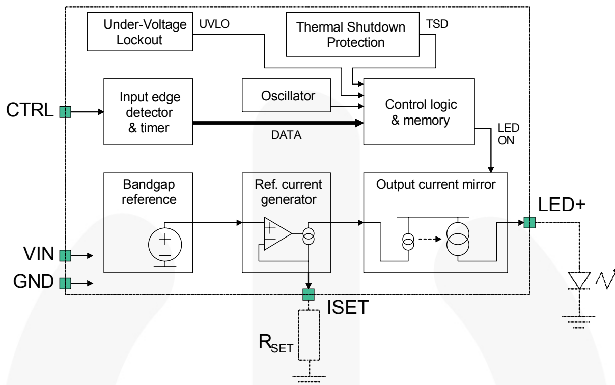
Figure 2. Block Diagram
