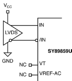
Figure 3e. LVDS Interface (AC-Coupled)
