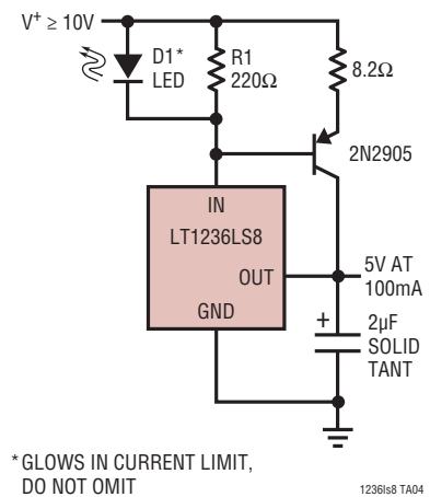
Boosted Output Current with Current Limit
