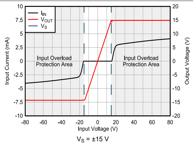
Figure 7-38. Input Current vs Input Overvoltage
