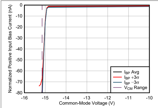
Figure 7-43. Positive Input Bias Current vs Common-Mode Voltage ( V_{S-} )
