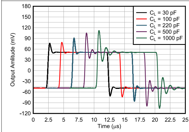
Figure 7-31. Small-Signal Response
