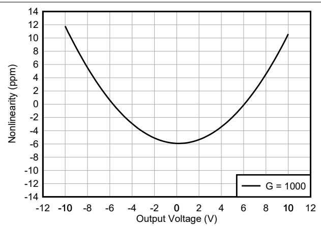
Figure 7-40. Gain Nonlinearity
