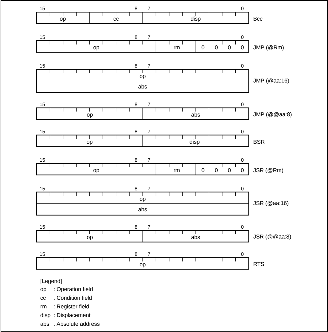
Figure 2.9 Instruction Formats of Branch Instructions
