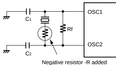
Negative resistor -R added (1) Negative resistor measurement circuit
