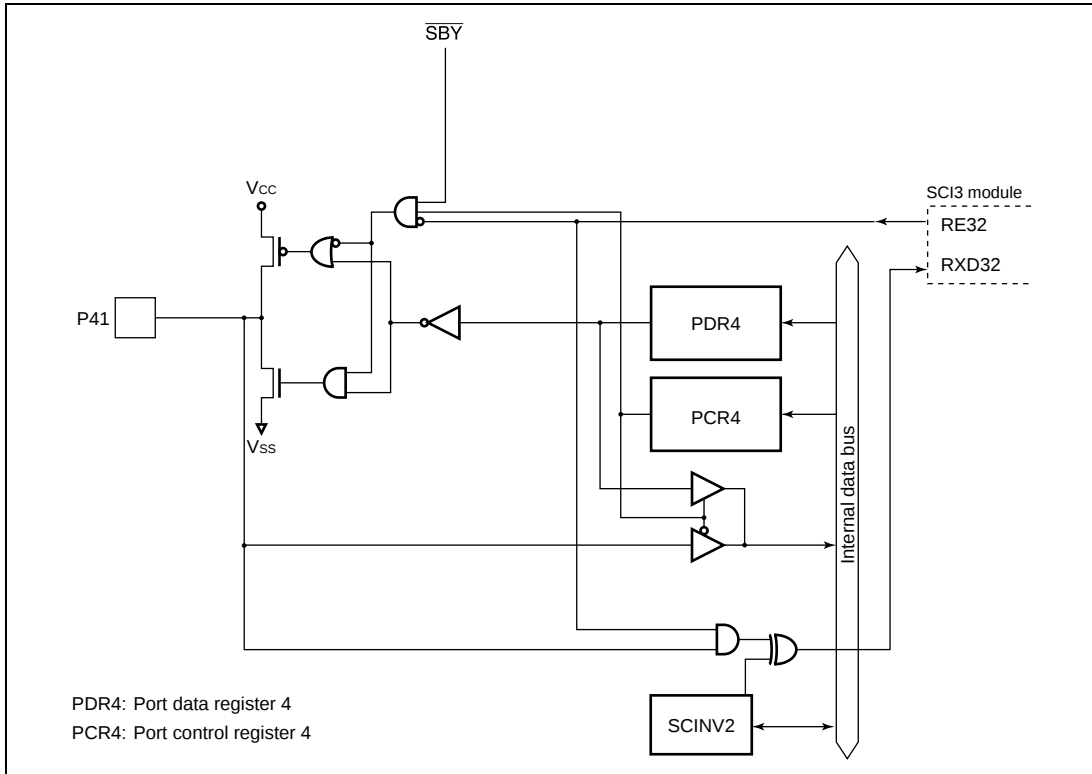
Figure B.2(c) Port 4 Block Diagram (Pin P41)
