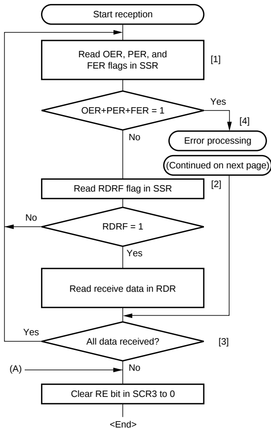
Figure 10.8 Sample Serial Data Reception Flowchart (Asynchronous Mode) (1)
