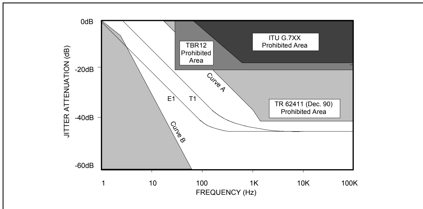
Figure 7-7. Jitter Attenuation
