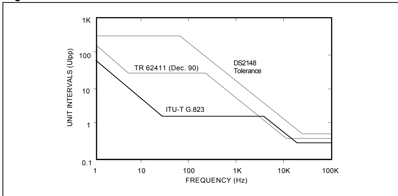
Figure 7-6. Jitter Tolerance
