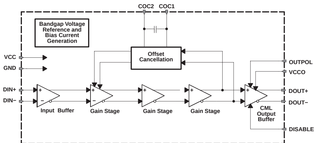
Figure 1. Block Diagram
