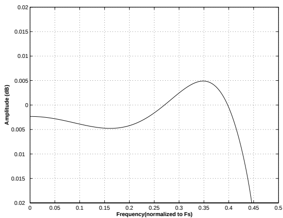
Figure 50. Double-Speed (fast) Passband Ripple
