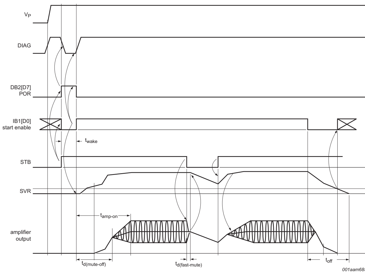
Fig 3. Start-up and shut-down in I 2 C mode
