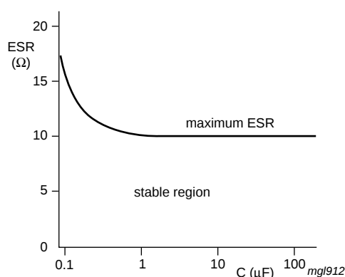
Fig 34. Curve for selecting the value of output capacitors for regulators 1 to 5
