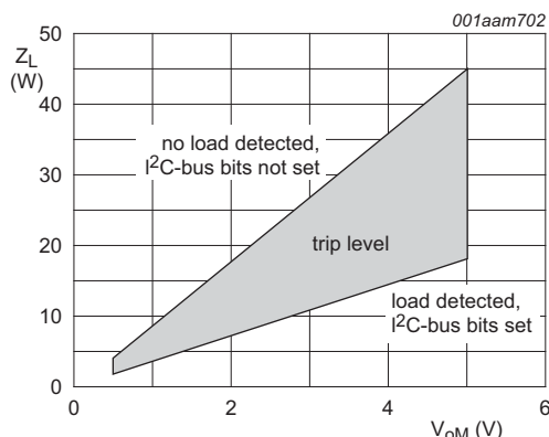
Fig 13. AC-load impedance as a function of peak output voltage (low current AC-load detection)
