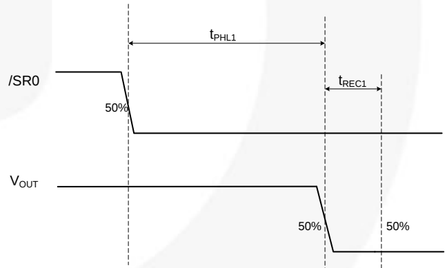
Figure 31. Reset Timing
