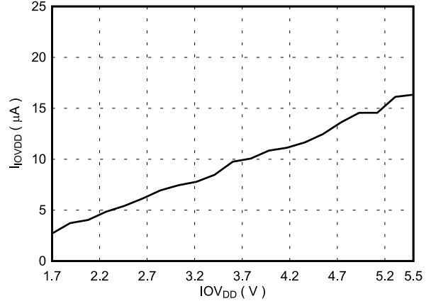
Figure 7-28. Supply Current ( IOV_{DD} ) vs Supply Voltage
