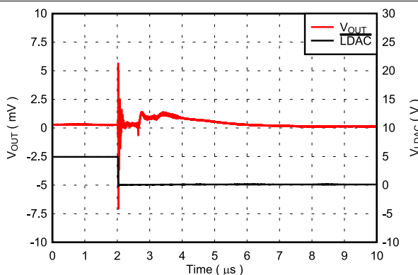
Figure 7-37. Glitch Impulse, 1 LSB Step, Falling Edge
