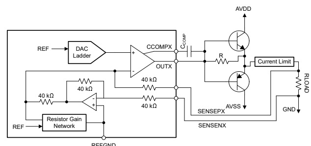
High Current Drive (1 A) Application
