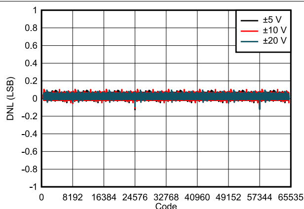
Figure 7-5. DAC81404 DNL vs Digital Input Code (Bipolar Outputs)
