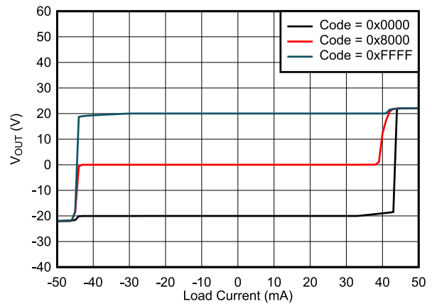
Figure 7-32. Source and Sink Capability
