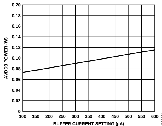
Figure 58. AVDD3 Power vs. Buffer Current Setting
