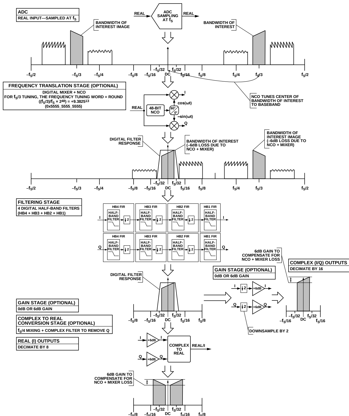
Figure 73. DDC Theory of Operation Example (Real Input, Decimate by 16)
