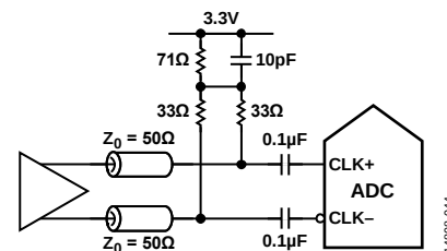
Figure 62. Differential CML Sample Clock
