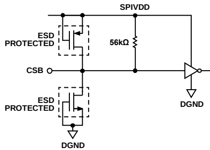
Figure 50. CSB Input
