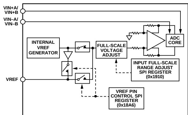
Figure 59. Internal Reference Configuration and Controls
