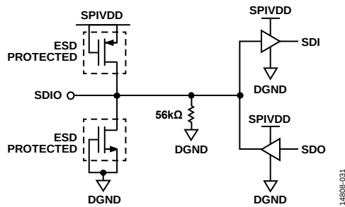
Figure 51. SDIO Input
