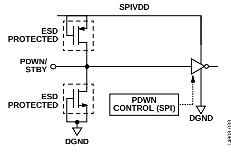
Figure 53. PDWN/STBY Input
