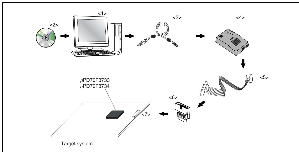
Figure A-3. System Configuration of On-Chip Emulation System
