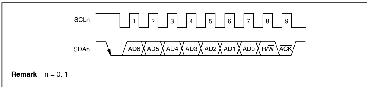
Figure 19-9. \overline{\text{ACK}}
