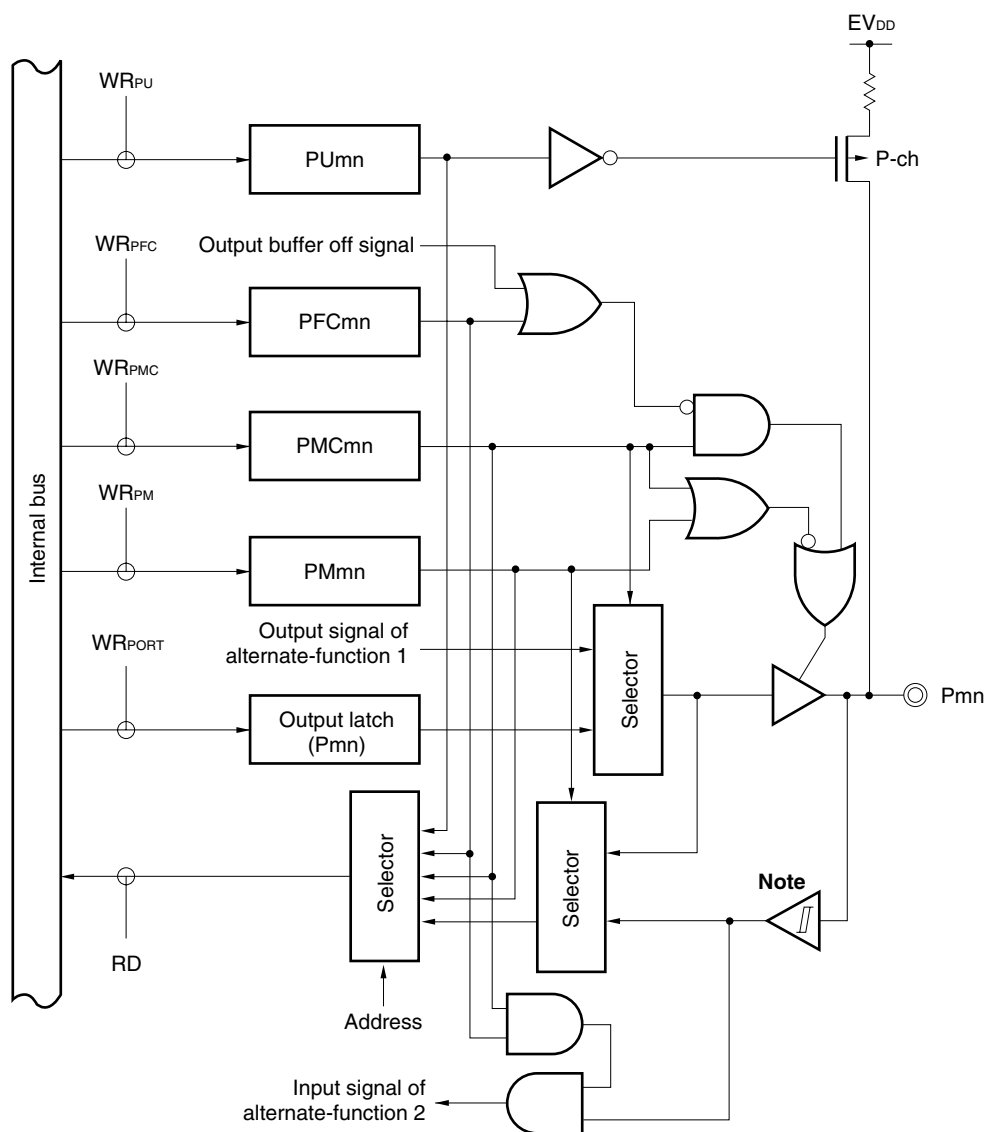
Figure 4-23. Block Diagram of Type E01-SULZ
