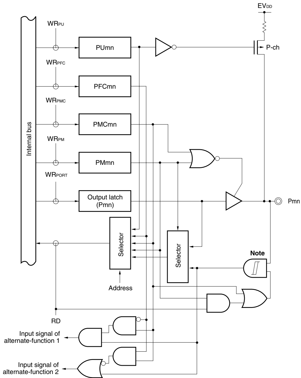
Figure 4-29. Block Diagram of Type E11-SULH
