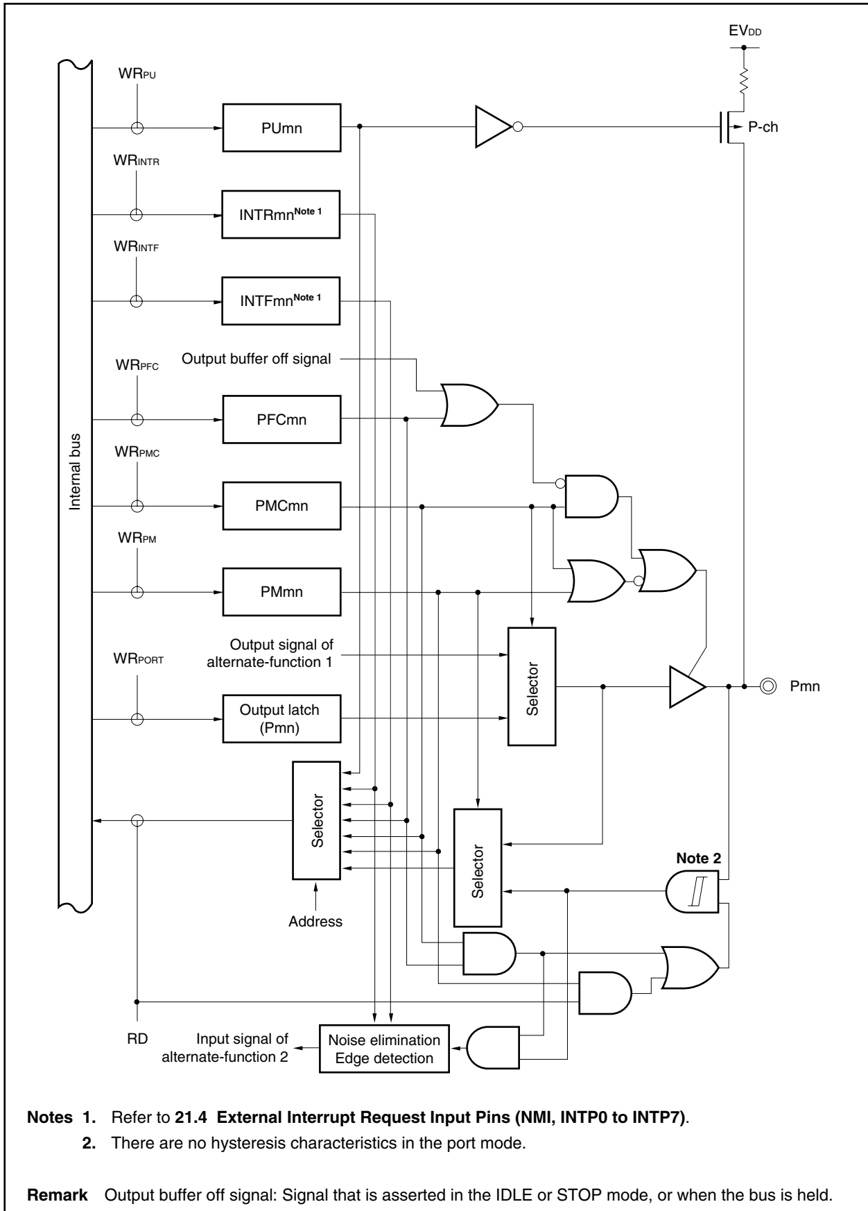
Figure 4-22. Block Diagram of Type E01-SUILZ
