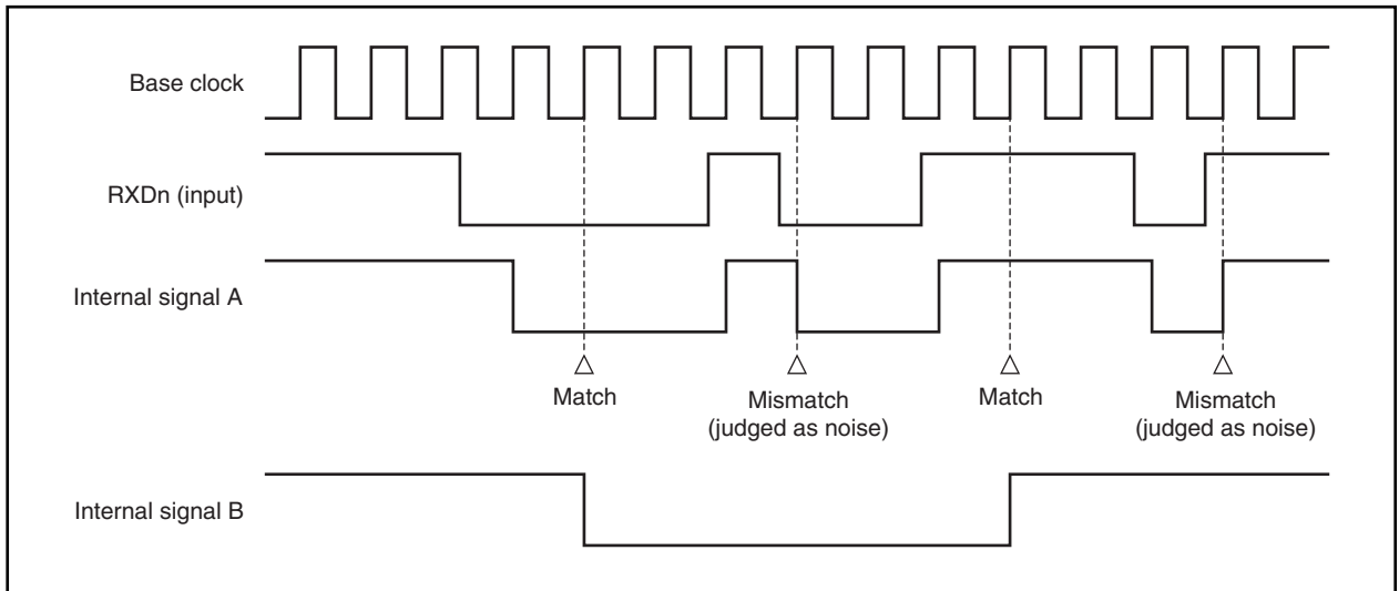
Figure 16-13. Timing of RXDn Signal Judged as Noise
