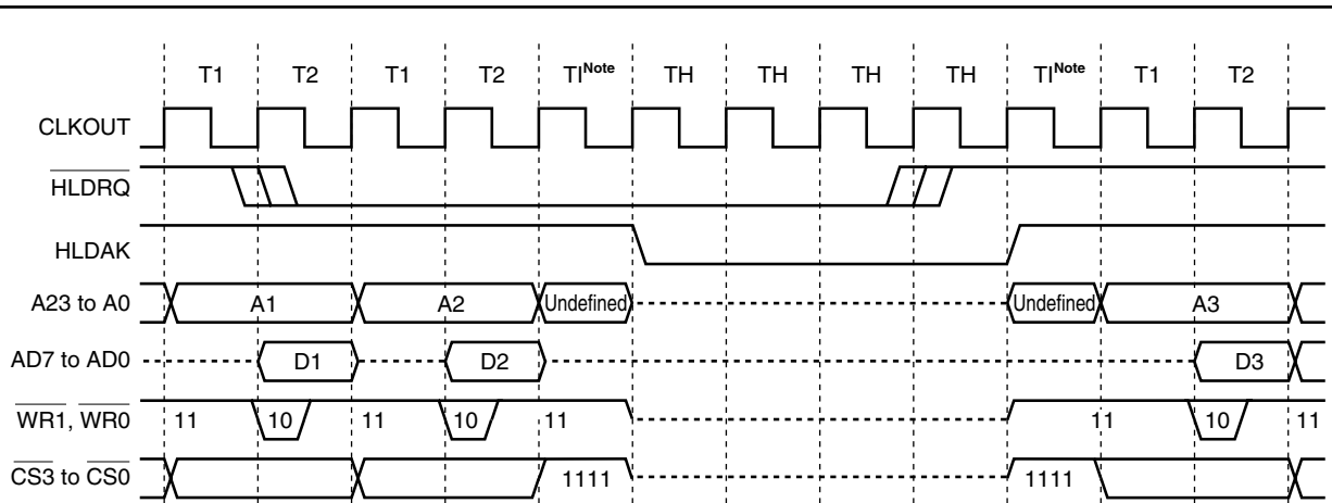
Figure 5-13. Separate Bus Hold Timing (Bus Size: 8 Bits, Write)
