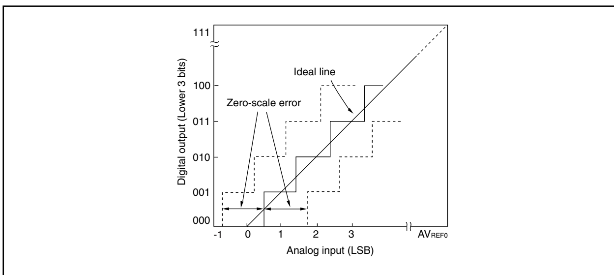
Figure 14-14. Zero-Scale Error
