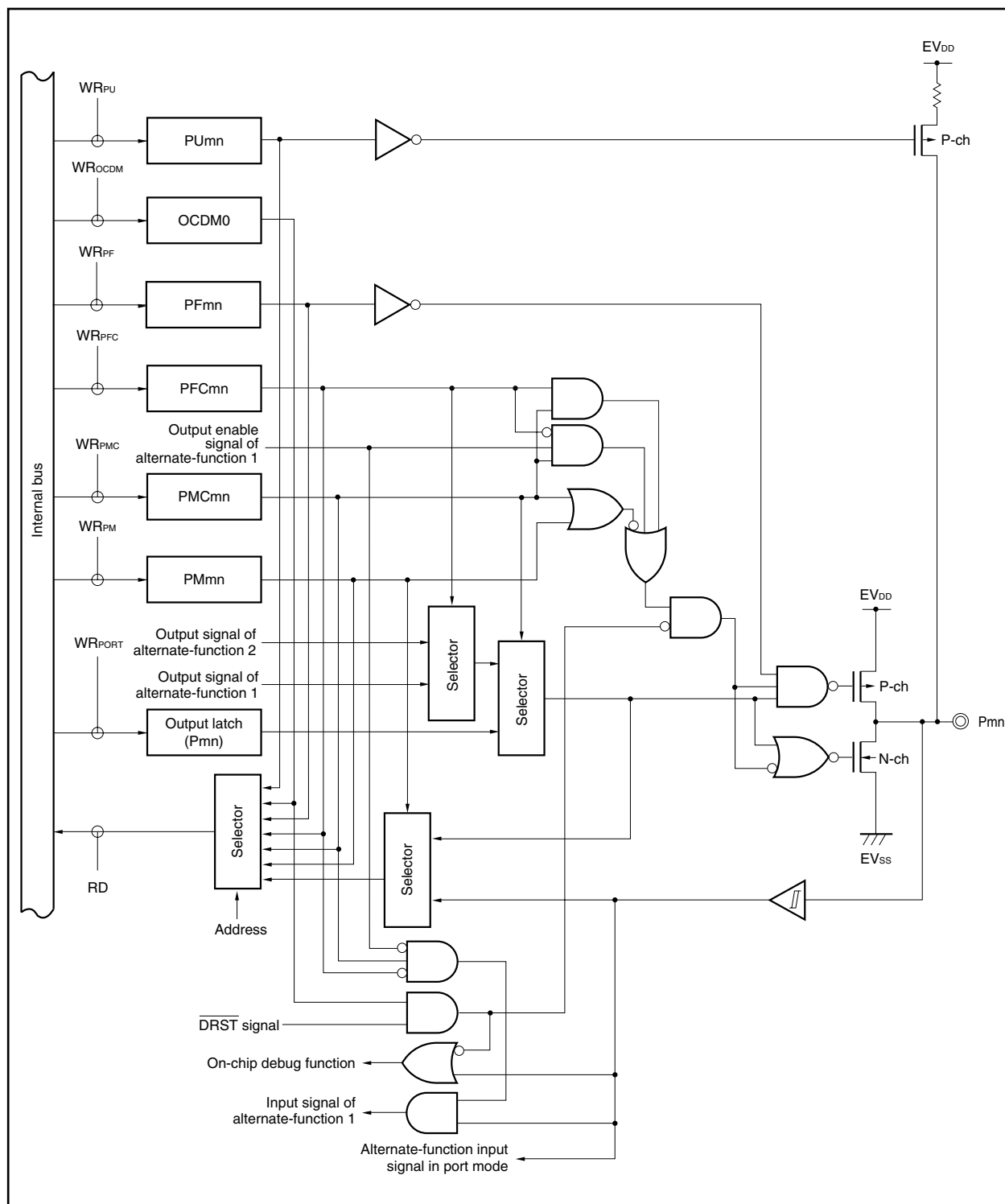
Figure 4-37. Block Diagram of Type OE201-SUFLT
