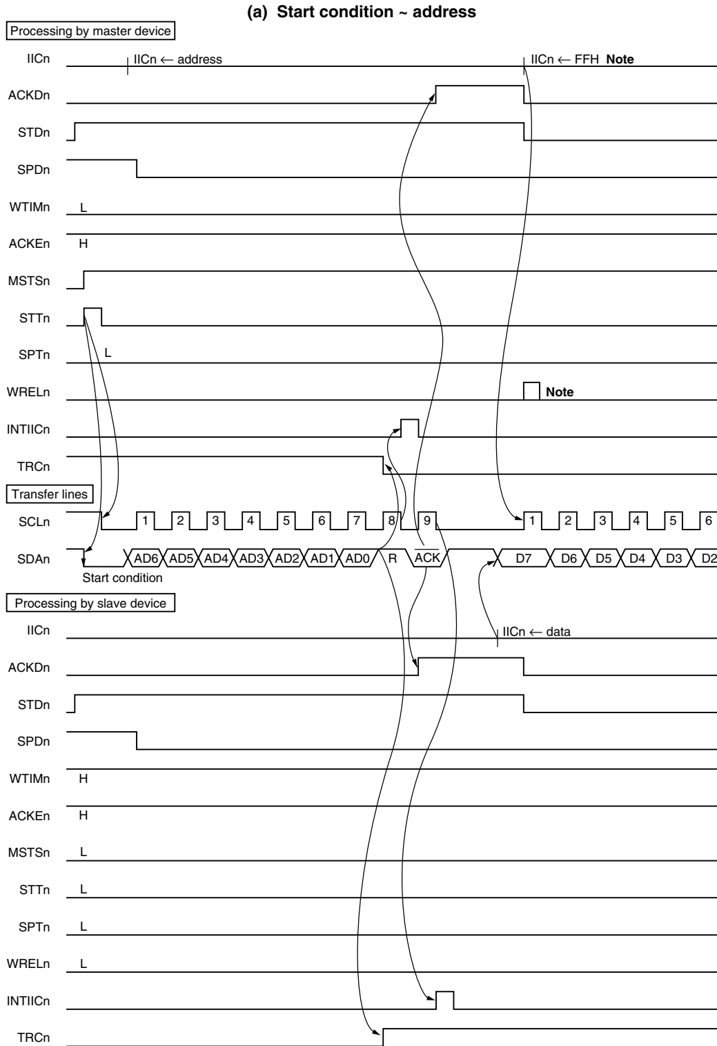
Figure 19-22. Example of Slave to Master Communication (When 8-Clock Wait for Master and 9-Clock Wait for Slave Are Selected) (1/3)
