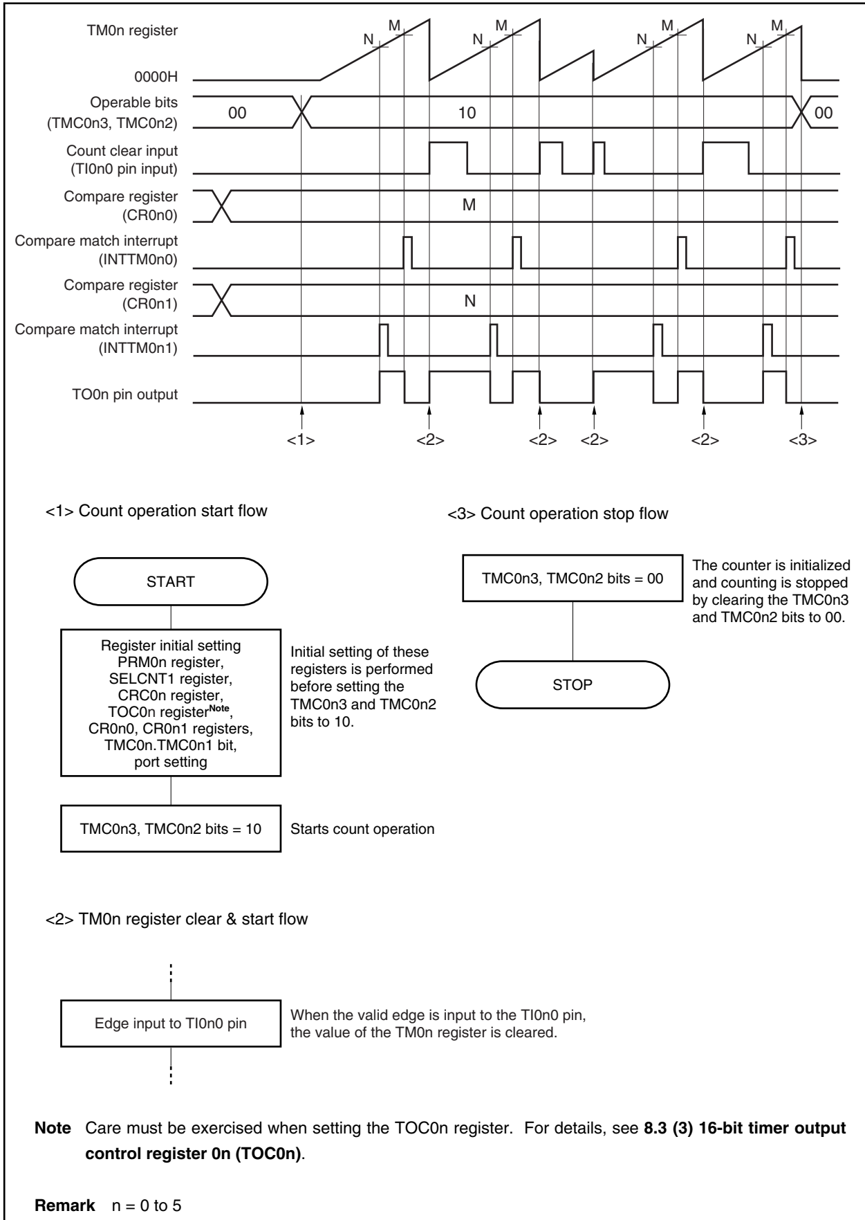
Figure 8-22. Example of Software Processing in Clear &amp; Start Mode Entered by TI0n0 Pin Valid Edge Input
