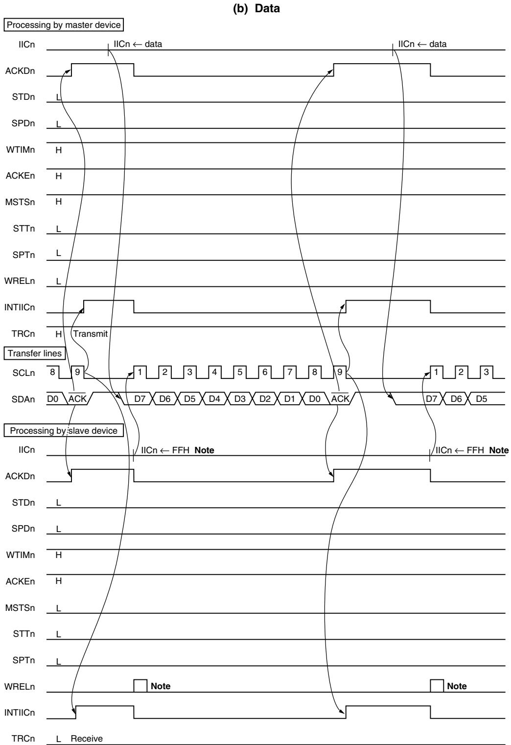
Figure 19-21. Example of Master to Slave Communication (When 9-Clock Wait Is Selected for Both Master and Slave) (2/3)
