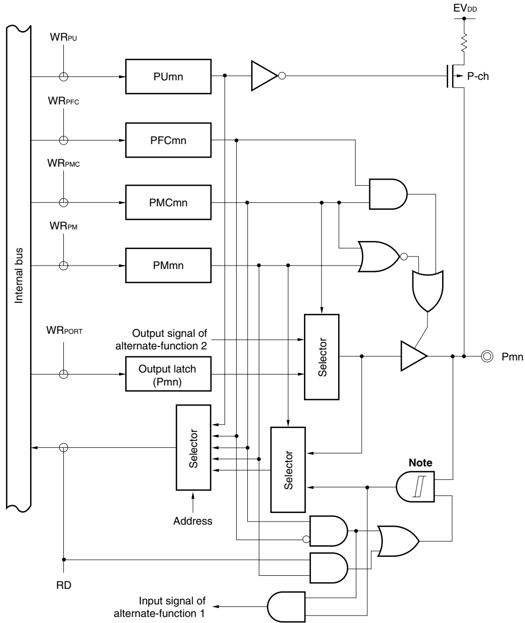
Figure 4-27. Block Diagram of Type E10-SUL
