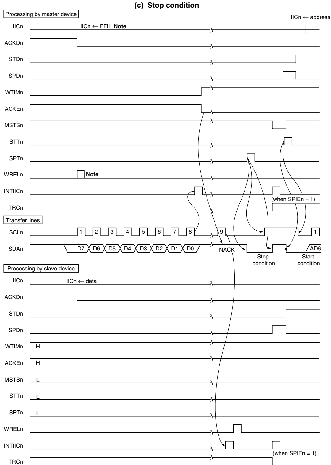
Figure 19-22. Example of Slave to Master Communication (When 8-Clock Wait for Master and 9-Clock Wait for Slave Are Selected) (3/3)
