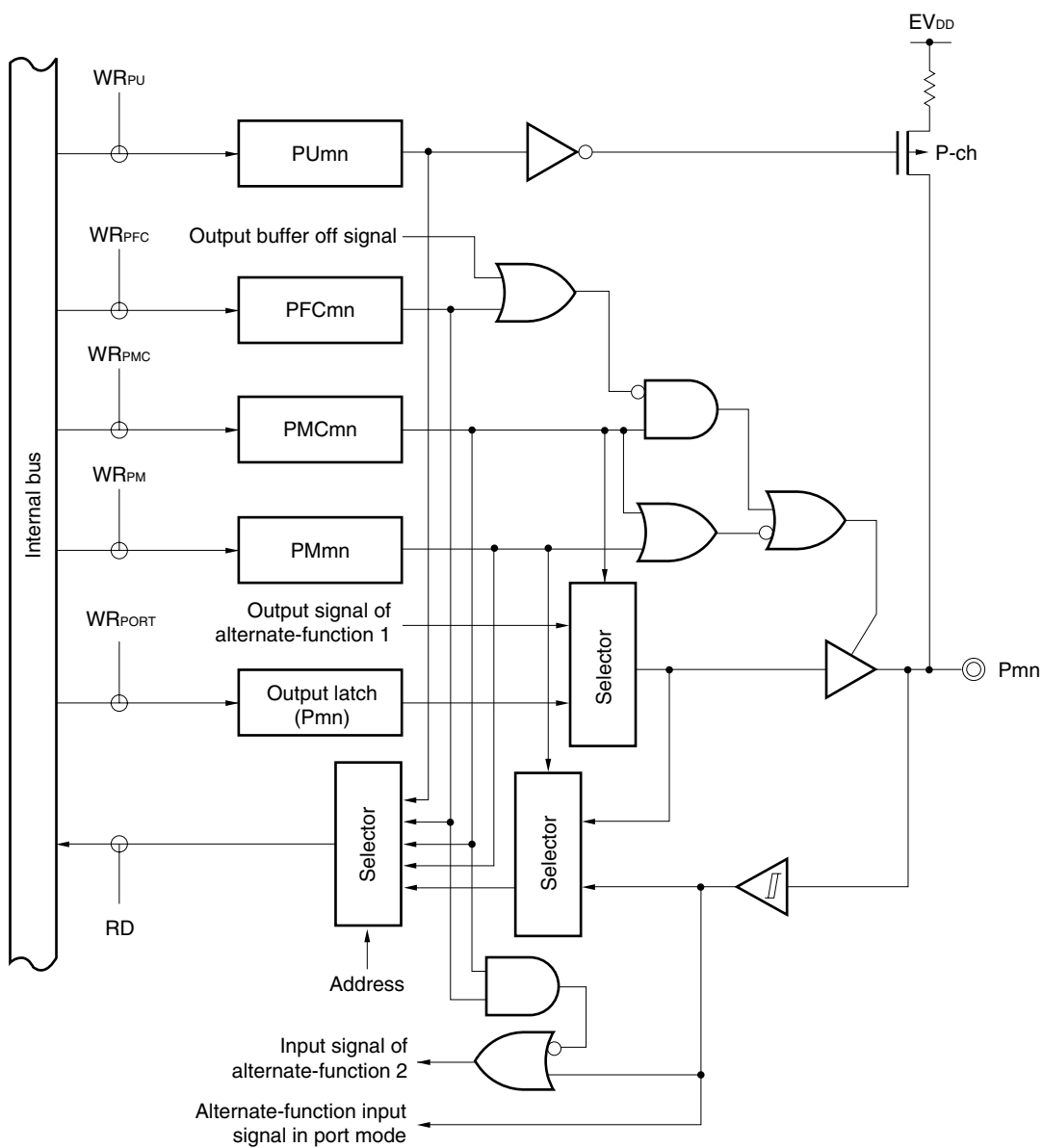
Figure 4-21. Block Diagram of Type E01-SUHTZ
