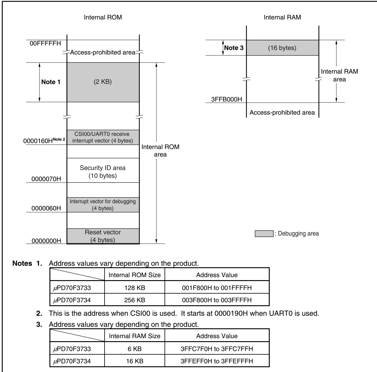
Figure 27-4. Memory Spaces Where Debug Monitor Programs Are Allocated
