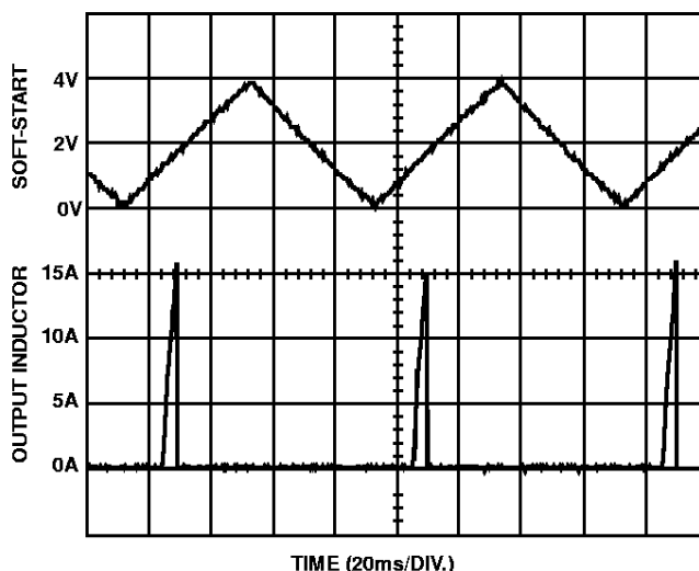
FIGURE 4. OVER-CURRENT OPERATION
