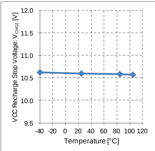
Figure 27. VCC Recharge Stop Voltage vs Temperature (BM2P131W-Z, BM2P141W-Z, BM2P151W-Z, BM2P181W-Z, BM2P201W-Z, BM2P241W-Z)
