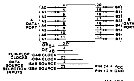
FUNCTIONAL DIAGRAM
