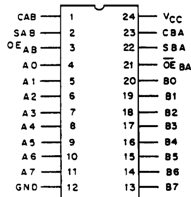
TERMINAL ASSIGNMENT
