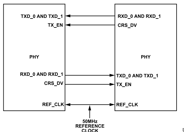
Figure 34. Back to Back with RMII Interface
