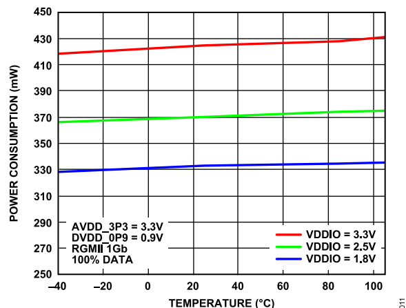
Figure 11. Power Consumption vs. Temperature, VDDIO Supply, 1 Gb, 100% Data
