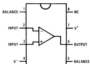
8LD Ceramic Dual-in Line Package
