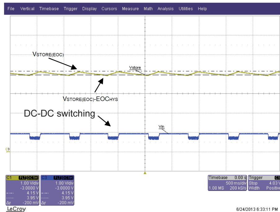
Figure 7. Triggering of V_{\text{EOC}} (BATT pin floating)
