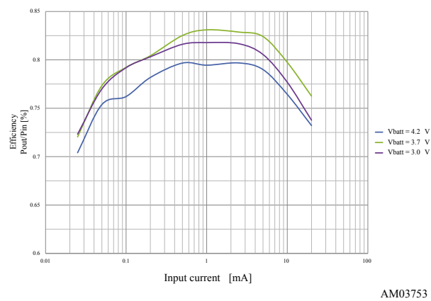
Figure 18. Efficiency vs. input current - V_{OC} = 15V
