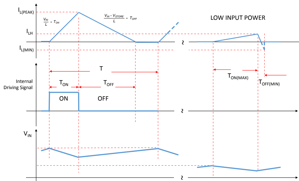
Figure 27. Inductor current and input voltage waveforms
