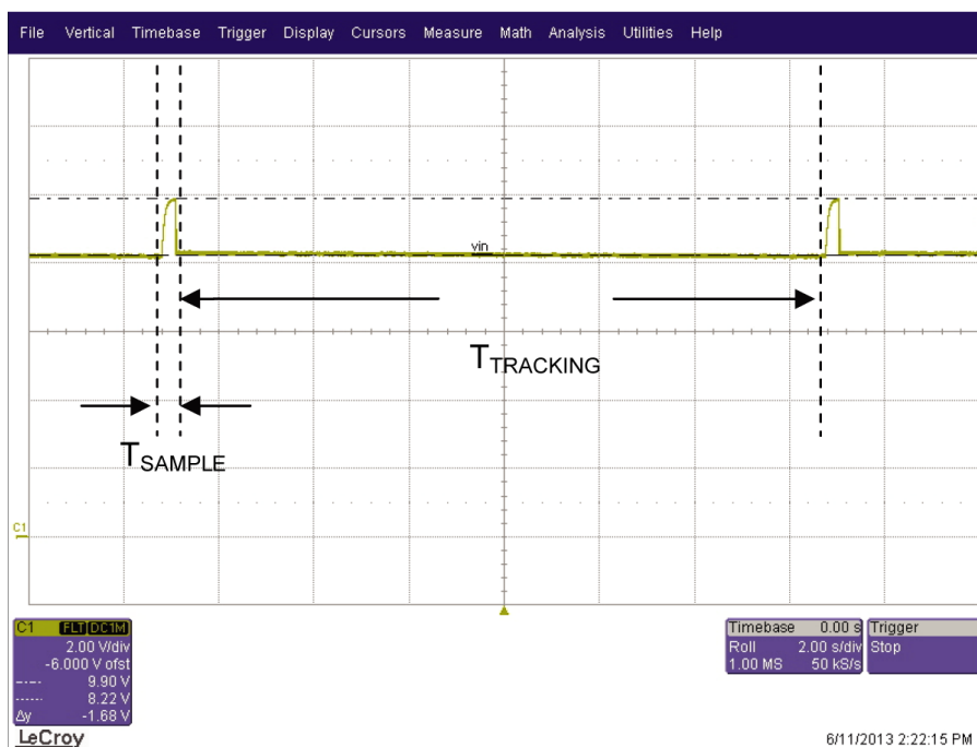
Figure 14. MPPT tracking
