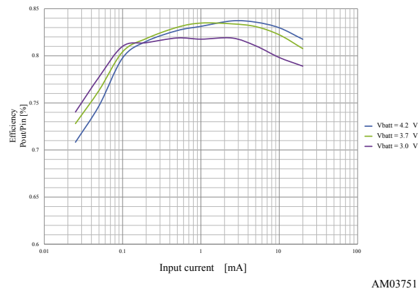
Figure 17. Efficiency vs. input current - V_{OC} = 12V
