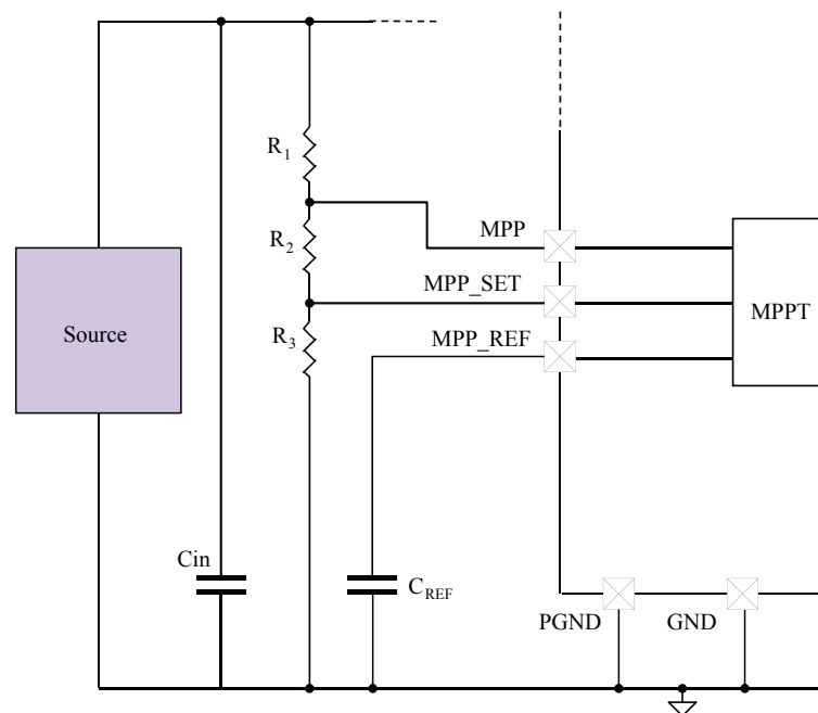
Figure 19. MPPT setup circuitry
