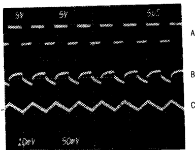
MAX741U SWITCHING WAVEFORMS – CONTINUOUS-CONDUCTION
