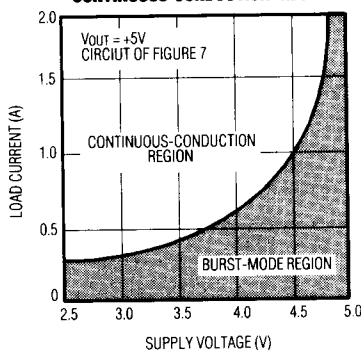
MAX741U STEP-UP CONTINUOUS-CONDUCTION REGION
