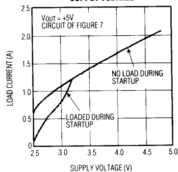
MAX741U STEP-UP LOAD CURRENT vs. SUPPLY VOLTAGE
