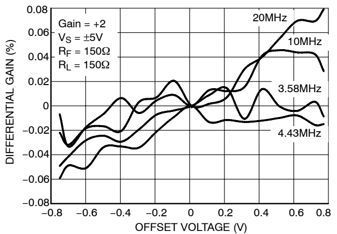
Figure 16. Differential Gain
