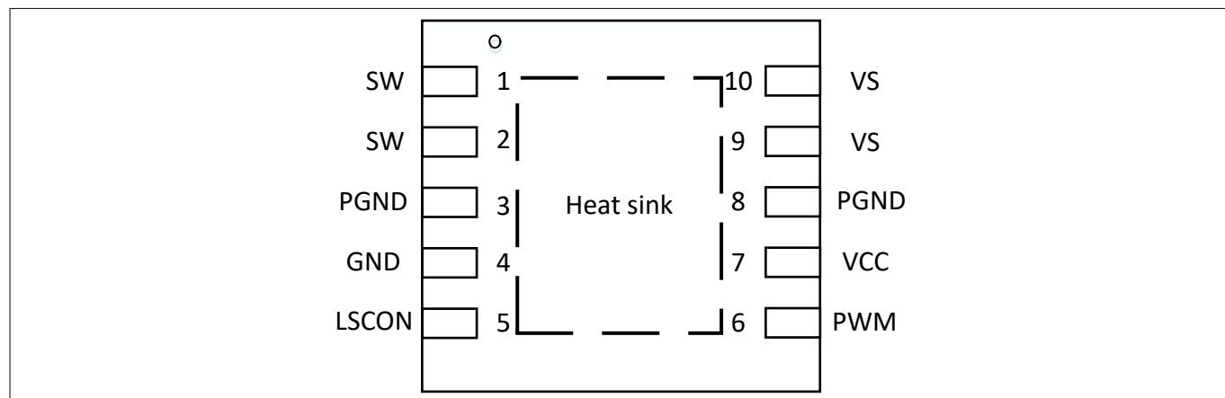
Figure 2 Pin configuration
