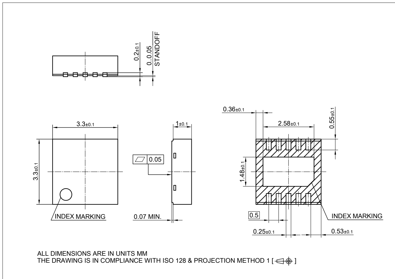
Figure 7 PG-TSON-10
