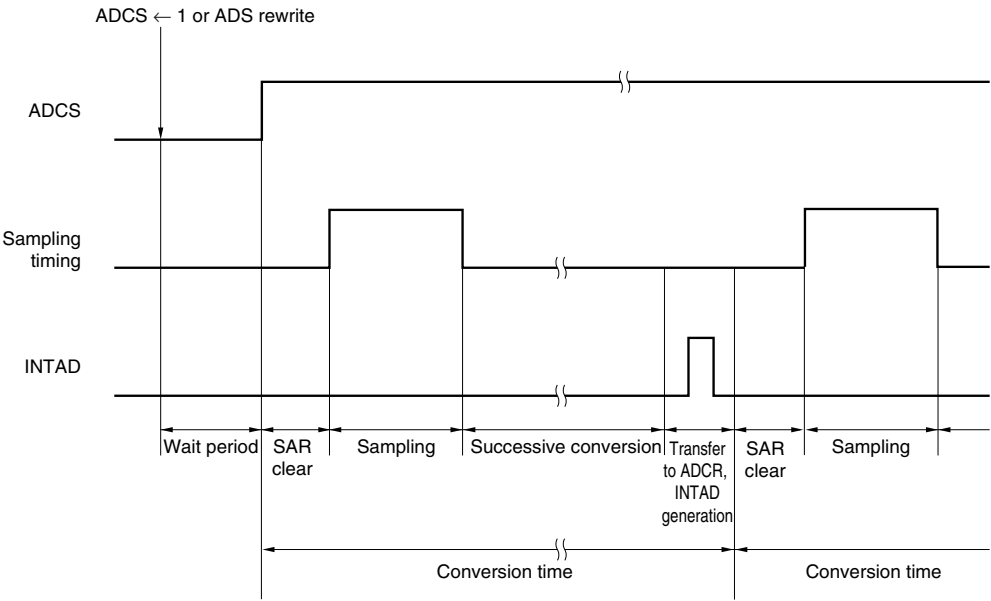
Figure 10-7. A/D Converter Sampling and A/D Conversion Timing
