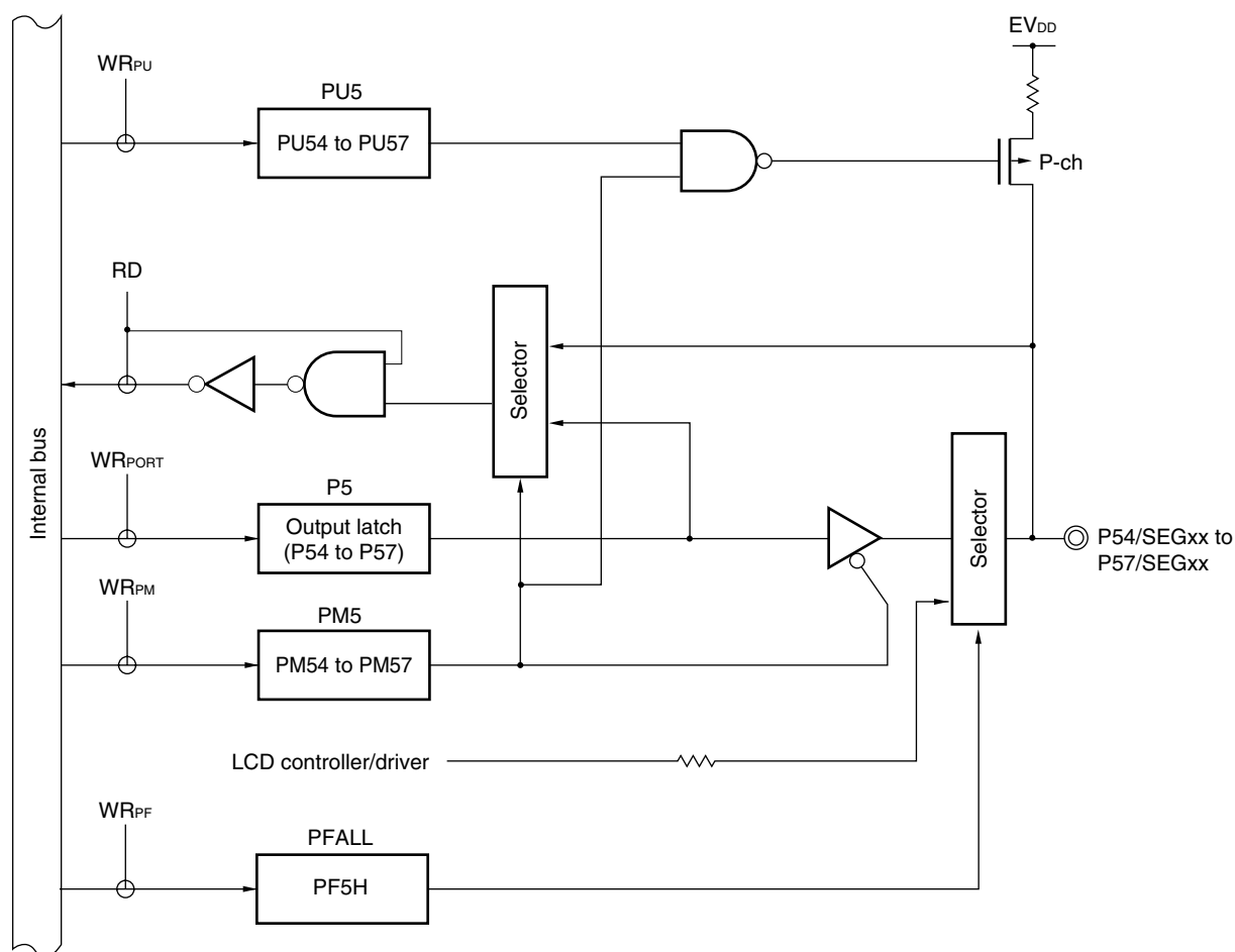
Figure 4-14. Block Diagram of P54 to P57
