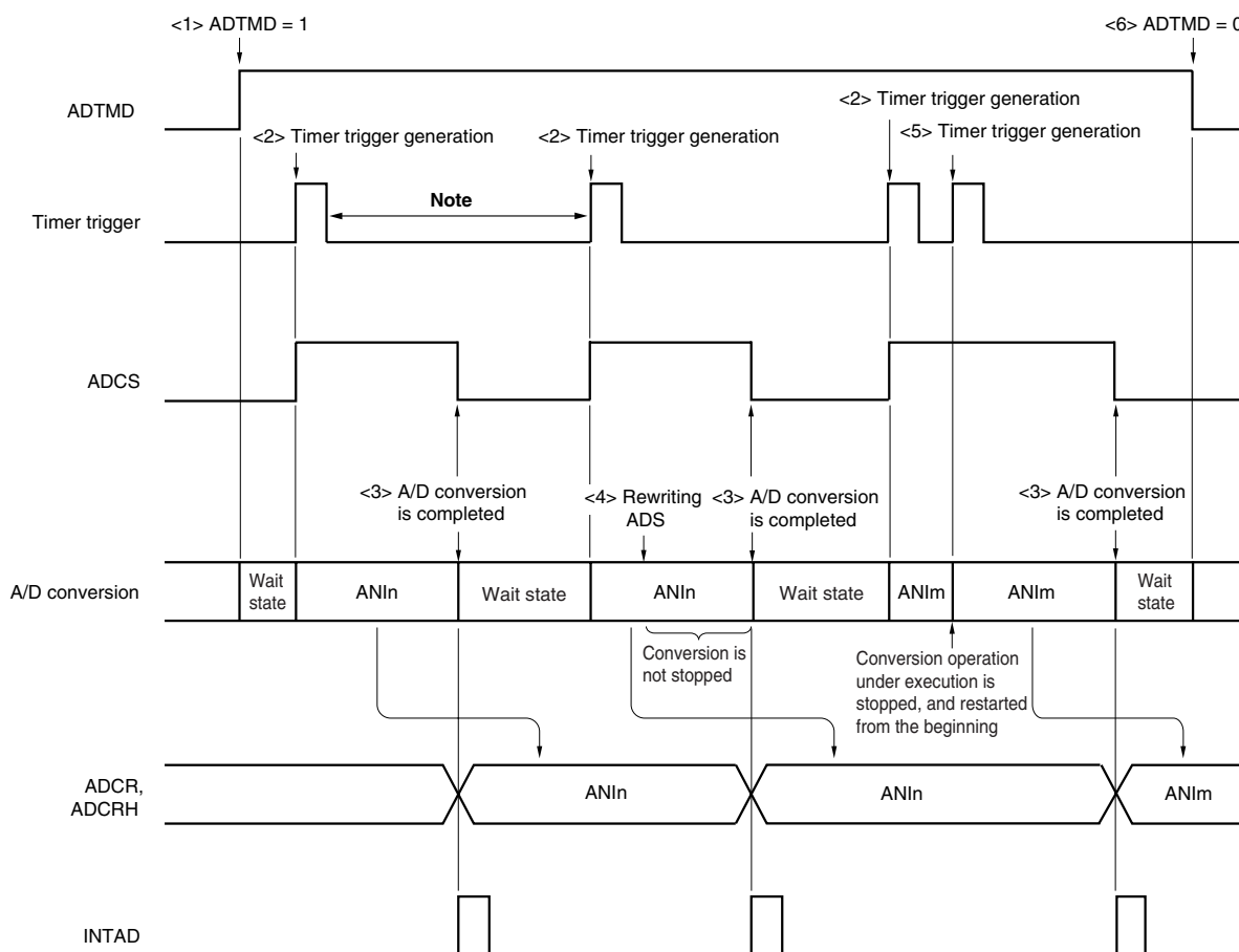
Figure 10-21. Timer trigger mode (Single conversion mode)
