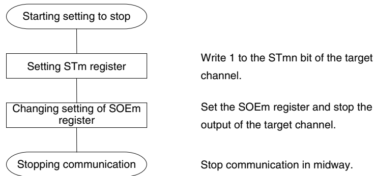
Figure 14-62. Procedure for Stopping Slave Transmission/Reception
