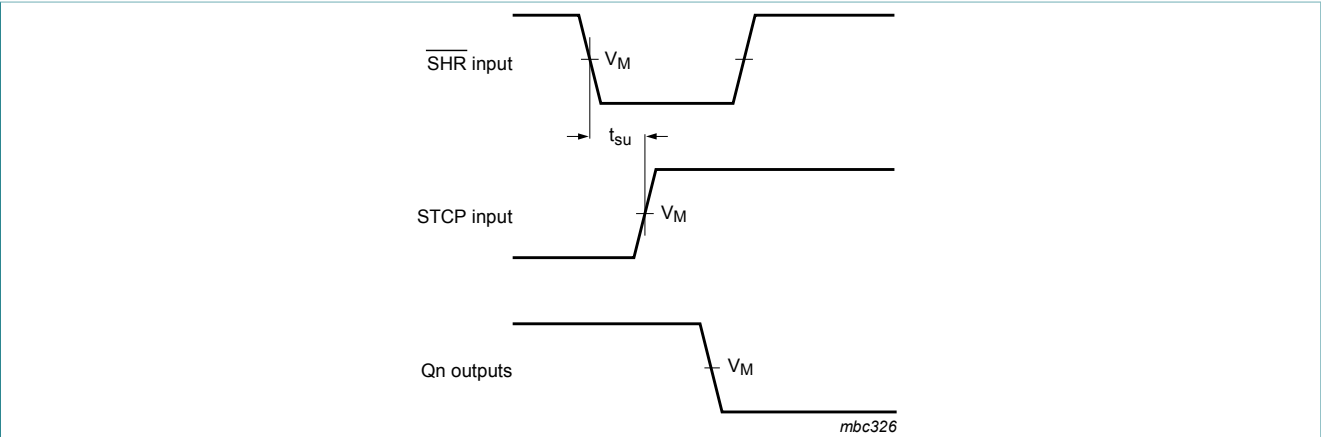
Measurement points are given in Table 8 . V_{OL} and V_{OH} are typical output voltage drops that occur with the output load. Figure 10. The shift reset (SHR) to storage clock (STCP) set-up times
