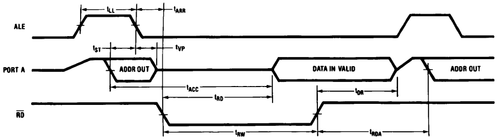
FIGURE 5. Read Cycle
