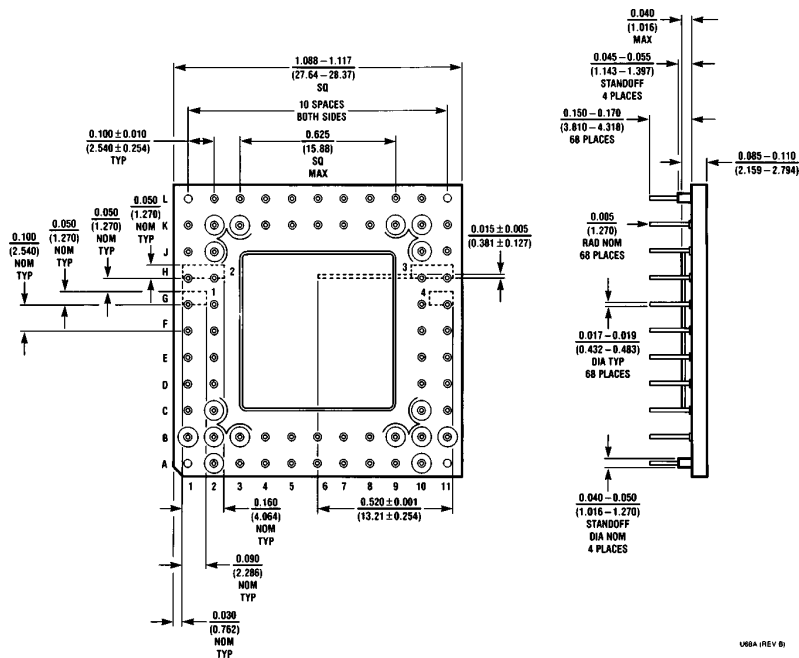
Pin Grid Array Pinout (U)
