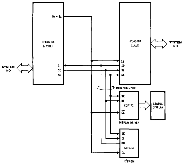
FIGURE 25. MICROWIRE/PLUS Application
