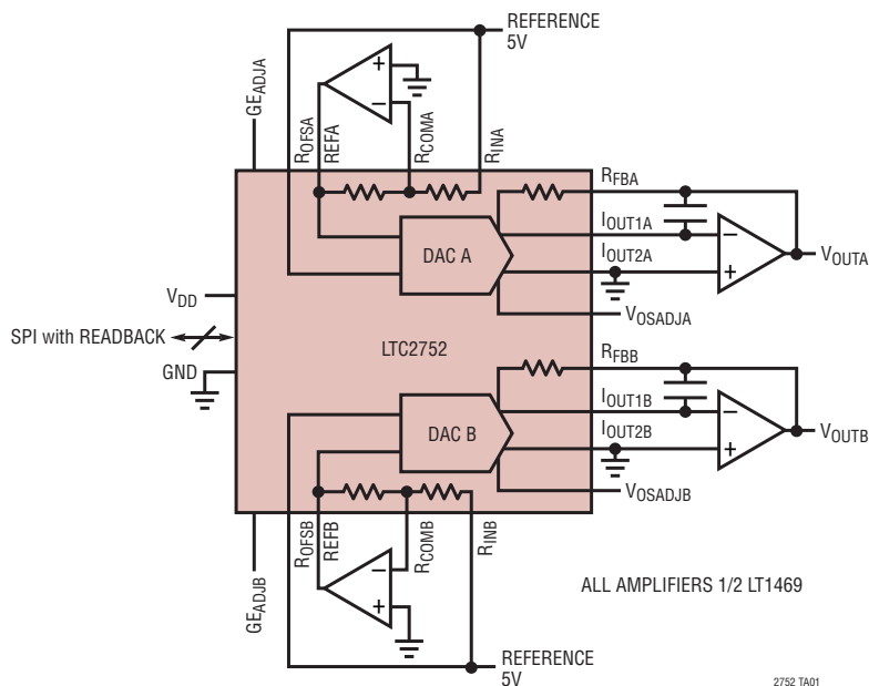
Dual 16-Bit V_{OUT} DAC with Software-Selectable Ranges
