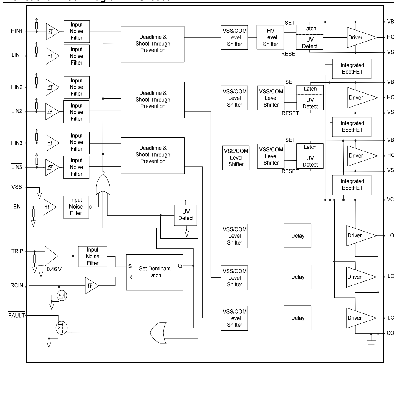
Functional Block Diagram: IRS23365D
