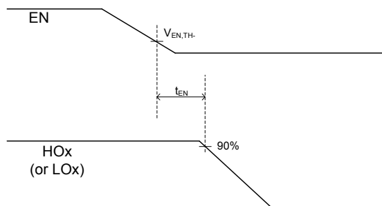
Figure 10: Output enable timing waveform
