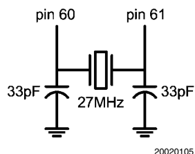
FIGURE 6. Crystal and Load Circuit
