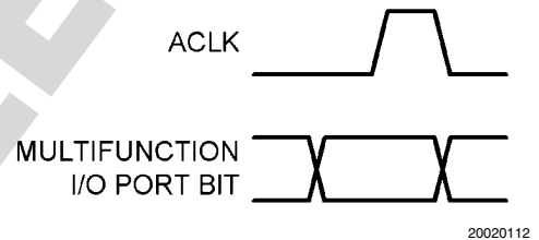
FIGURE 5. I/O Port Data Write Timing
