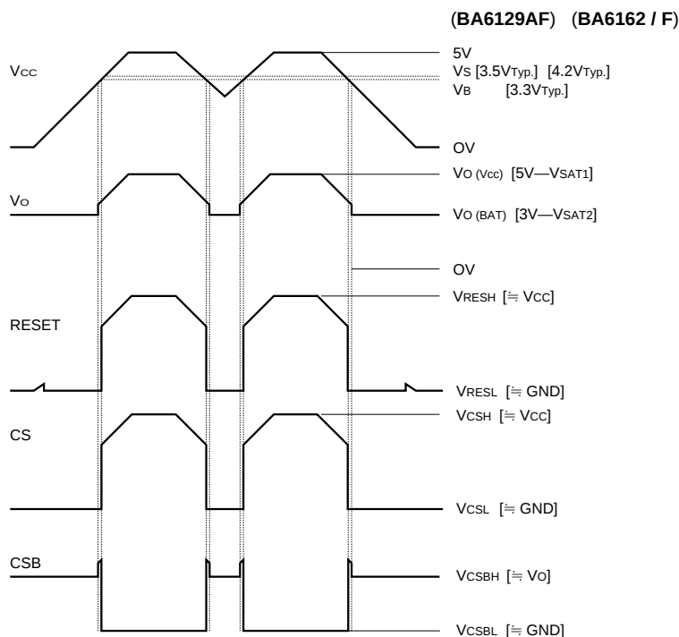
Fig. 2 Timing chart
