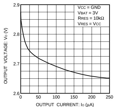
Fig. 15 Output voltage vs. output current ( I ) (when using battery backup)
