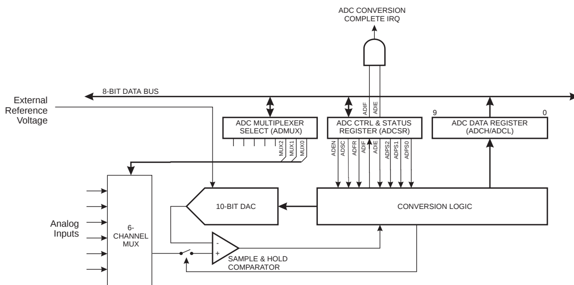
Figure 44. Analog to Digital Converter Block Schematic
