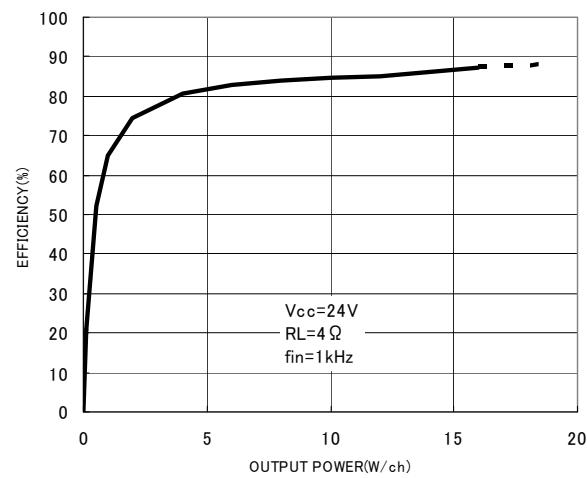
Fig.20 Output power—Efficiency ( R_L=4\Omega )
