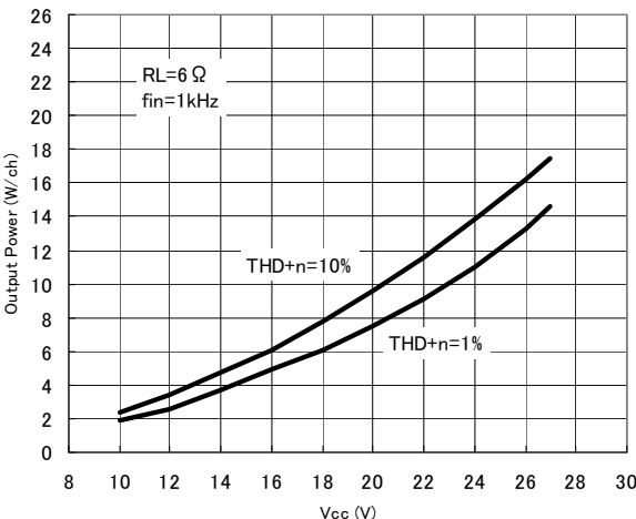
Fig.16 Power supply voltage—Output power (RL=6Ω)
