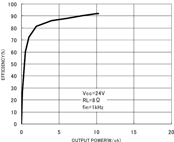
Fig.14 Output power—Efficiency (RL=8Ω)
