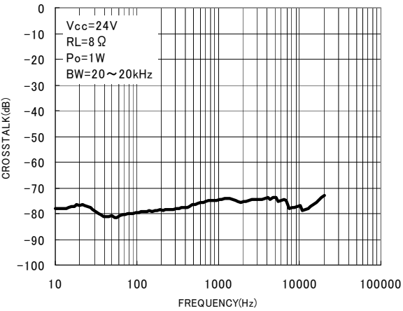
Fig.6 Frequency—Crosstalk
