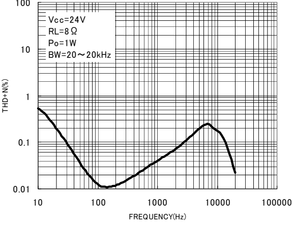
Fig.4 Frequency—THD+N
