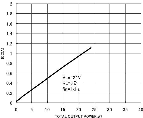
Fig.18 Total output power—Current consumption (RL=6Ω)
