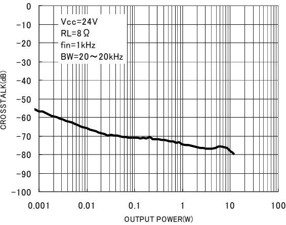
Fig.5 Output power—Crosstalk
