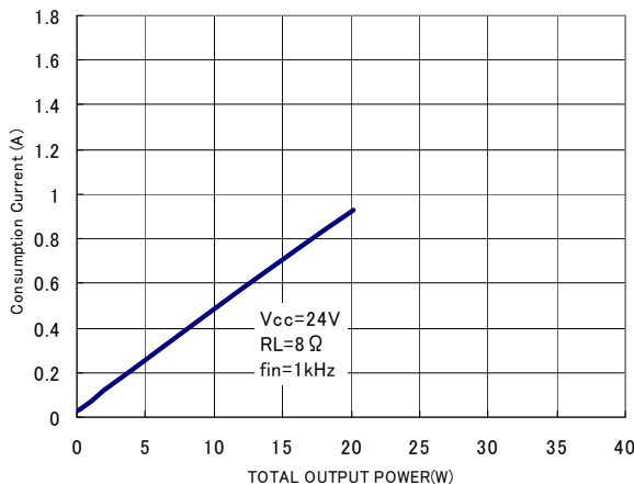
Fig.15 Total output power—Current consumption (RL=8Ω)
