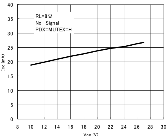
Fig. 2 Power supply voltage—Current consumption
