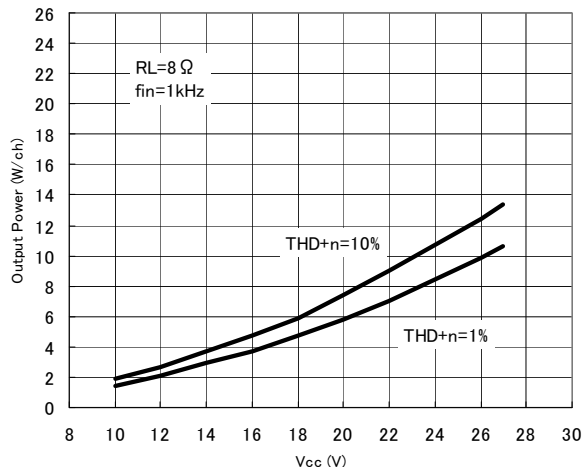
Fig.13 Power supply voltage—Output power (RL=8Ω)
