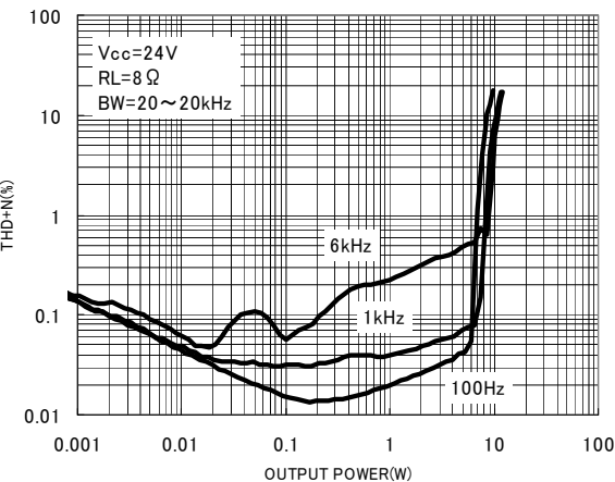
Fig.3 Output power—THD+N
