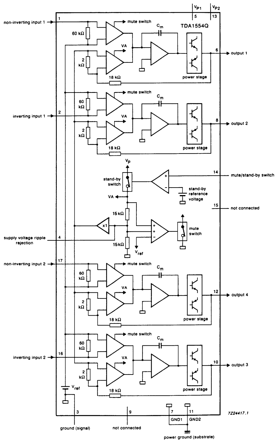
Fig.1 Block diagram.
